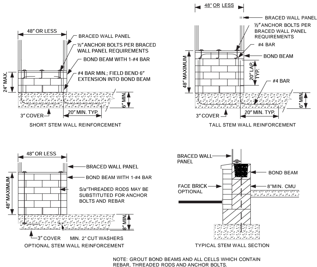
FIGURE R602.10.7 MASONRY STEM WALLS SUPPORTING BRACED WALL PANELS
