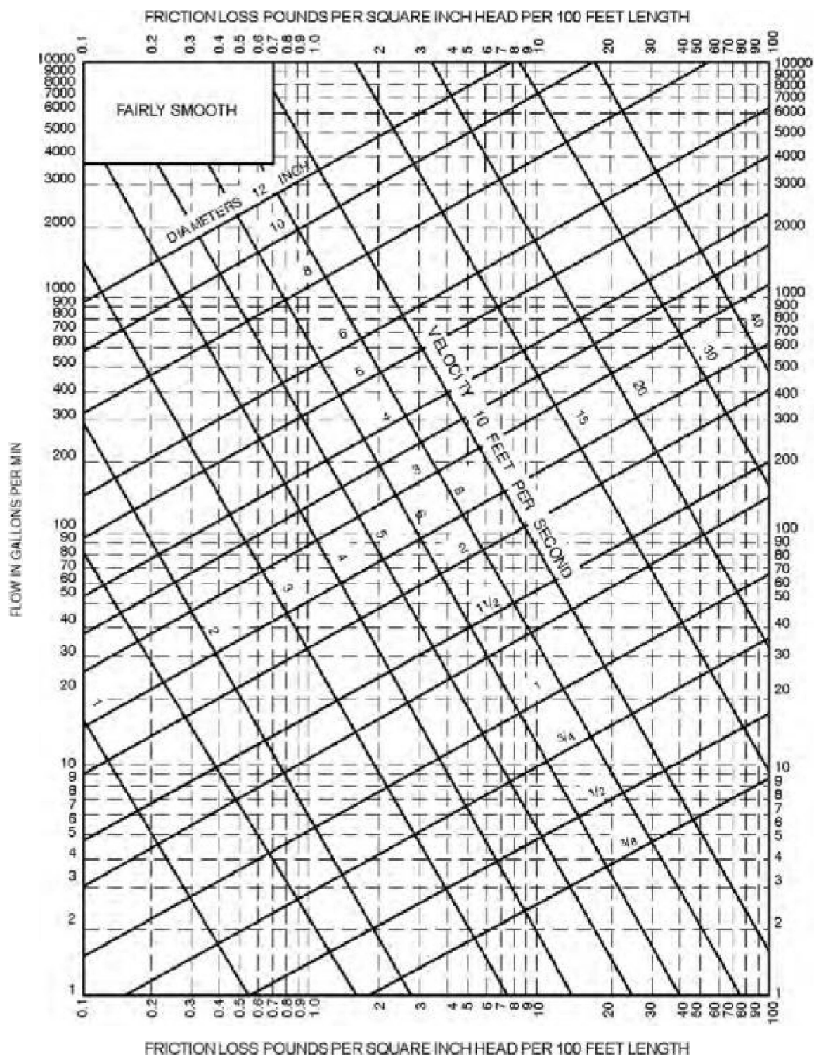
FIGURE AP103.3(5) FRICITION LOSS IN FAIRLY SMOOTH PIPE a
