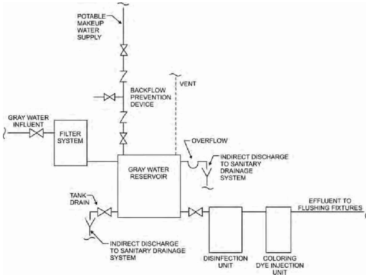
FIGURE AOI01.1 (1) GRAY WATER RECYCLING SYSTEM FOR FLUSHING WATER CLOSETS AND URINALS
