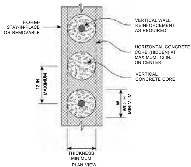
FIGURE R611.3(3) SCREEN-GRID WALL SYSTEM
