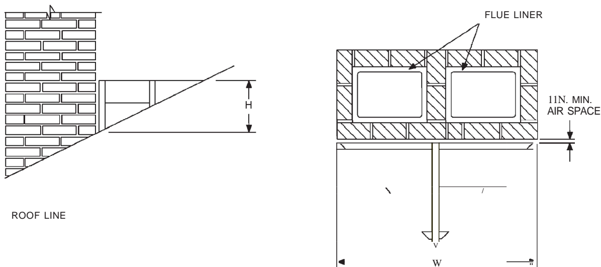
FIGURE R1003.18 CLEARANCE FROM COMBUSTIBLES
