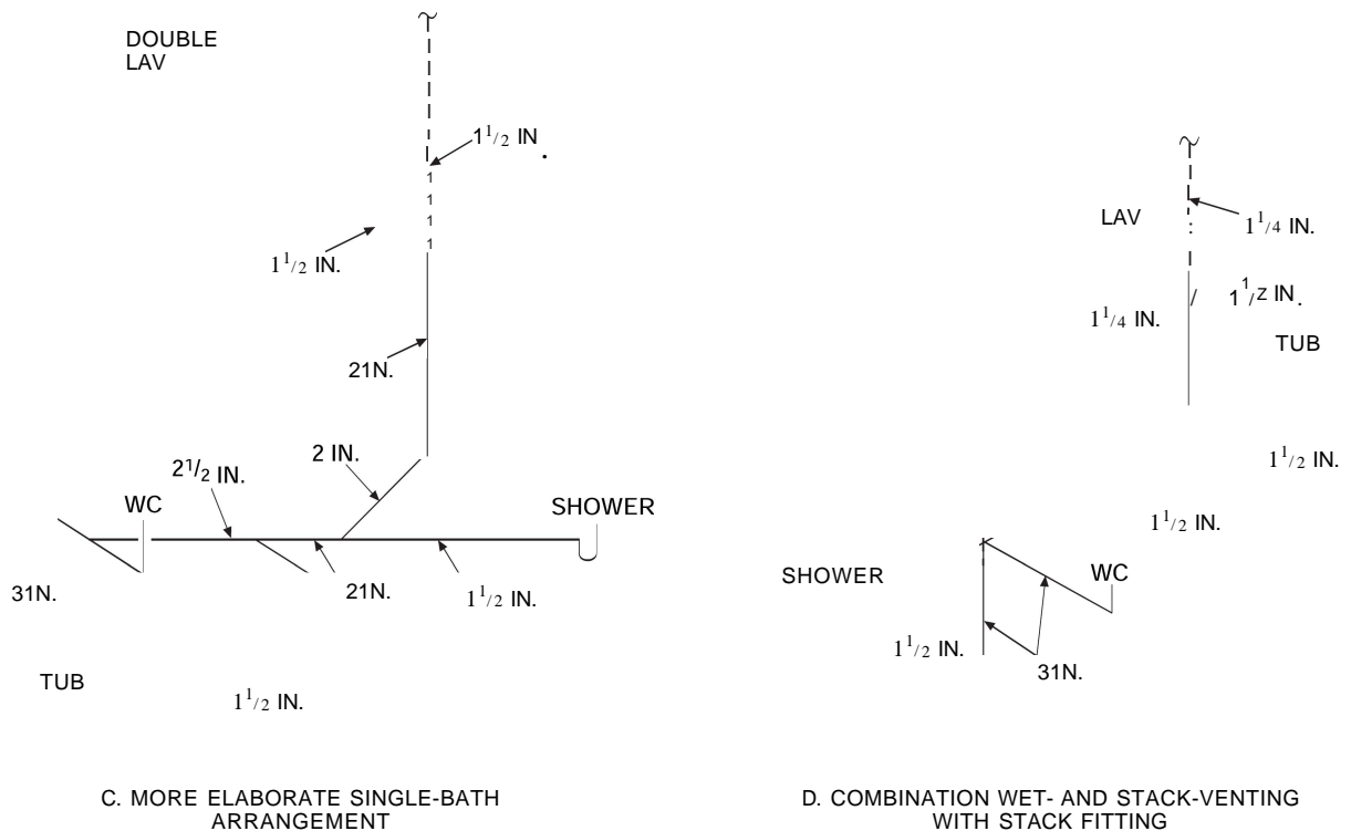
FIGURE N1 TYPICAL SINGLE-BATH WET-VENT ARRANGEMENTS
