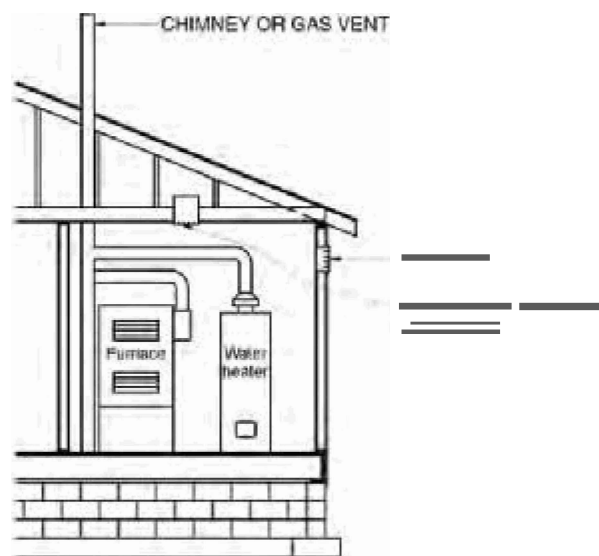
FIGURE G2407.6.2 (304.6.2) SINGLE COMBUSTION AIR OPENING, ALL AIR FROM OUTDOORS (see Section 2407.6.2)
