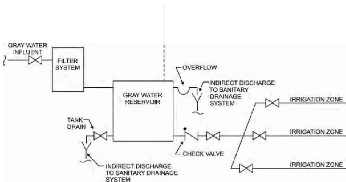
FIGURE AOI01.1 (2) GRAY WATER RECYCLING SYSTEM FOR SUBSURFACE LANDSCAPE IRRIGATION
