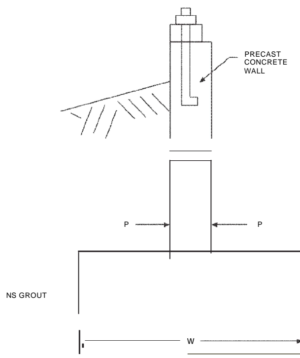
FIGURE R403.4(2) BASEMENT OR CRAWL SPACE WITH PRECAST FOUNDATION WALL ON SPREAD FOOTING
