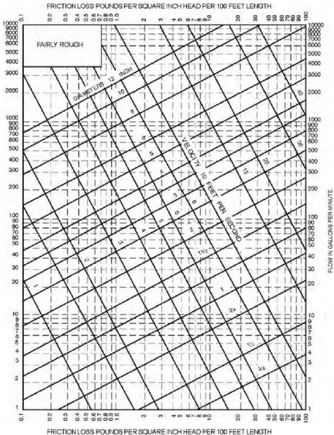
FIGURE AP103.3(6) FRICTION LOSS IN FAIRLY ROUGH PIPE a
