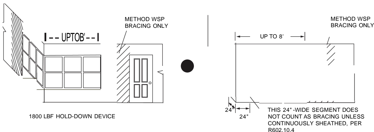
FIGURE R602.10.1.4.1 BRACED WALL PANELS AT ENDS OF BRACED WALL LINES IN SEISMIC DESIGN CATEGORIES Do, D1 AND D2
