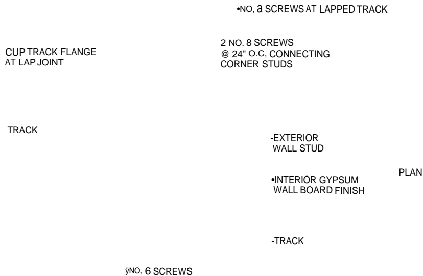
FIGURE R603.3.5 TRACK SPLICE
