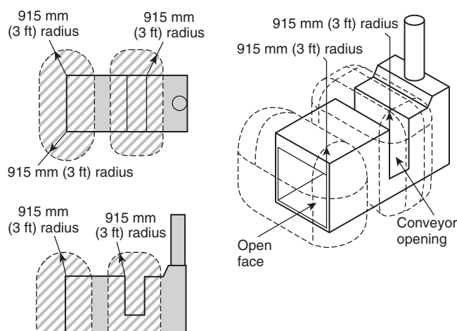
FIGURE 43.1.4.4.2 Class I, Division 2; Class I, Zone 2; Class II, Division 2; or Zone 22 Locations Adjacent to an Open-Face or Open-Front Spray Booth or Spray Room. [33:Figure 6.5.2]
