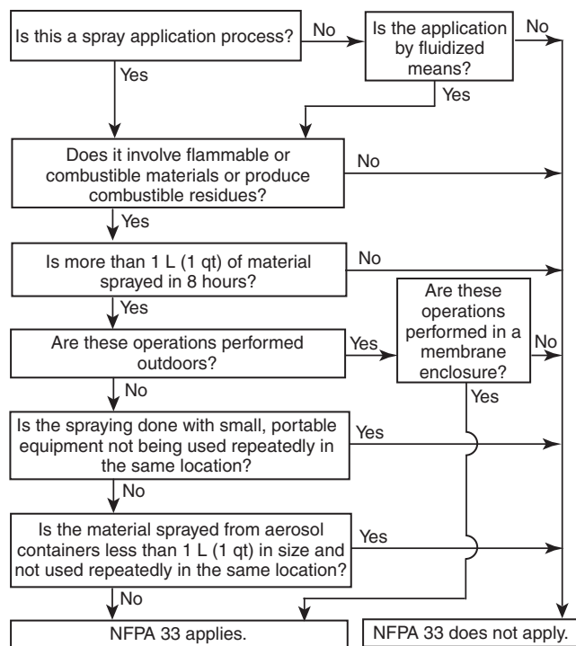
Δ FIGURE A.43.1.1.1 Decision Tree — Does Chapter 43 Apply? [33:Figure A.1.1.1]
