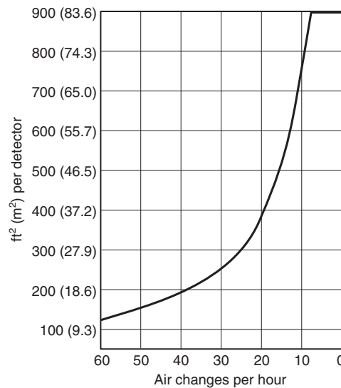
■ FIGURE 13.7.4.3.8.2.2 High Air Movement Areas (Not to Be Used for Under-Floor or Above-Ceiling Spaces). [72:Figure 17.7.6.3.3.2]
