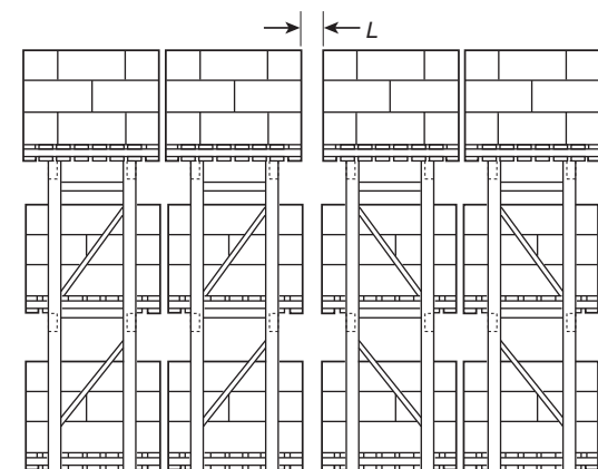
FIGURE A.34.7.3.1(e) Automatic Storage-Type Rack.
