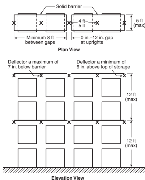
FIGURE 66.16.1.1(a) Single-Row Rack Sprinkler Layout for Design Scheme "A." [30: Figure 16.6.1.1(a)]
