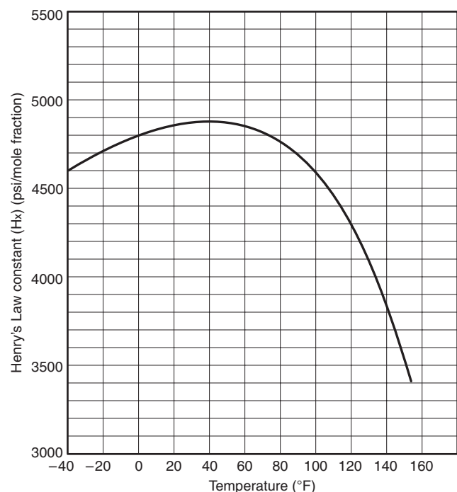
FIGURE E.1.1(a) Henry's Law Constant for Nitrogen Solubility in Liquid Halon 1301.
