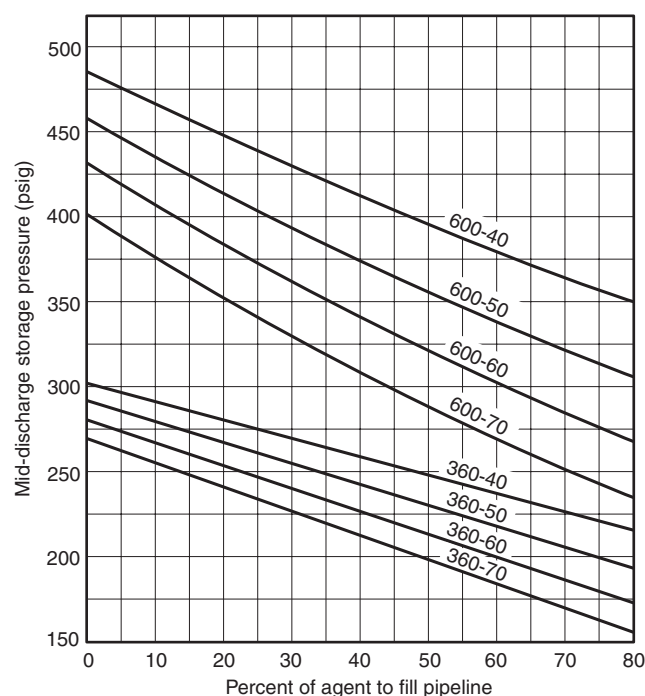
FIGURE H.1(e) Percent of Agent to Fill Pipeline.
