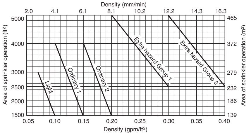
FIGURE 11.2.3.1.1 Density/Area Curves.
