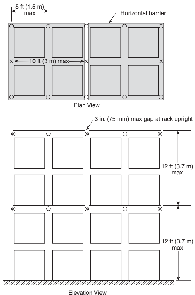
FIGURE 17.1.2.9.4.2(A) Alternative Protection Double-Row Racks.
