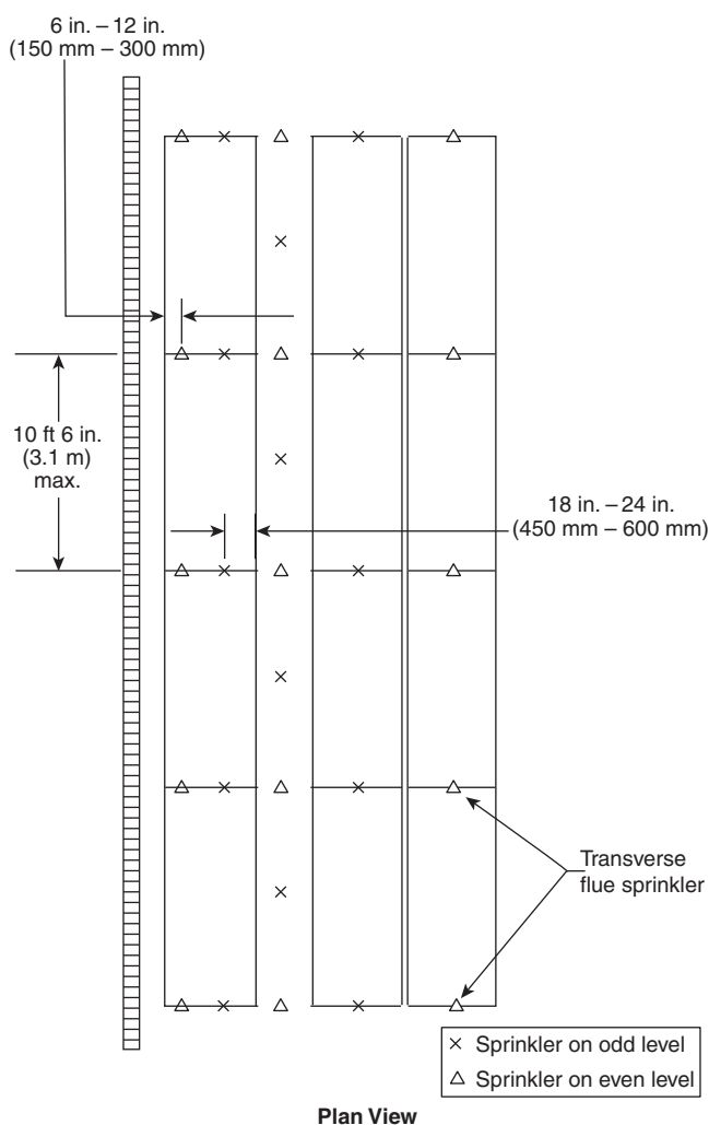
FIGURE 20.5.6.4 Sprinkler Location and Spacing in Transverse Flues.
