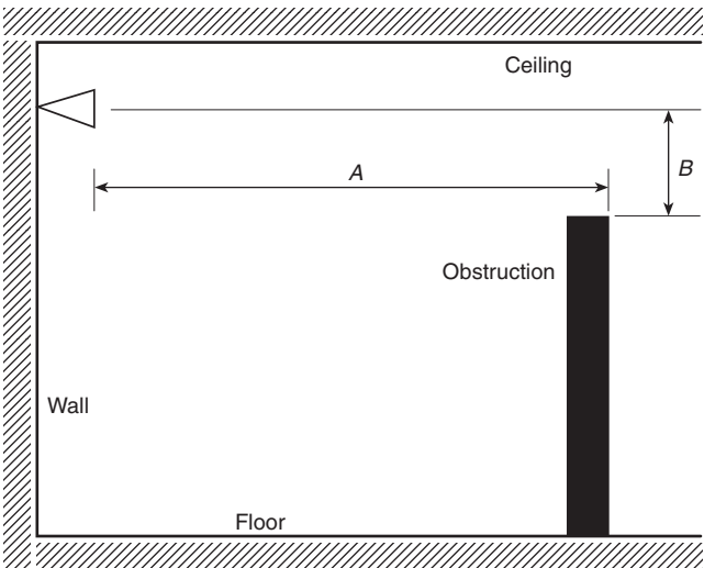
FIGURE 8.9.5.2.2 Suspended or Floor-Mounted Obstruction (Extended Coverage Sidewall Sprinklers) in Light Hazard Occupancy Only.
