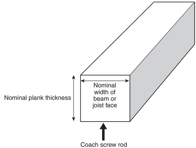
FIGURE 9.1.5.7.2 Dimensions for Structural Members with Coach Screw Rods.
