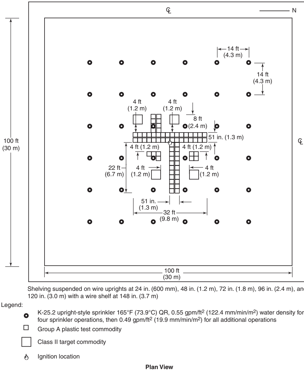
FIGURE A.20.3(e) Fire Test A6 — Plan View.
