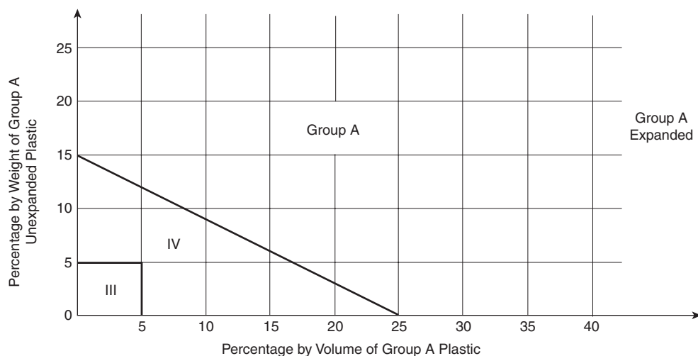
FIGURE 5.6.3.3.3(a) Commodities Containing a Mixture of Expanded and Unexpanded Group A Plastics.
