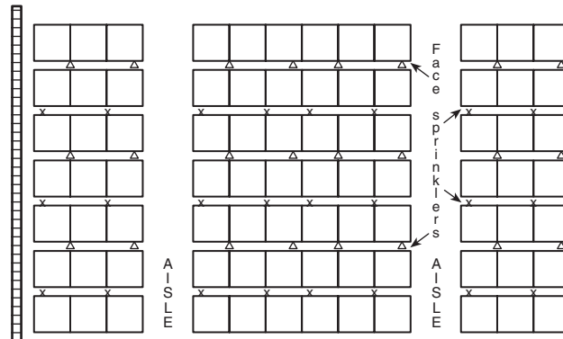
Elevation View
