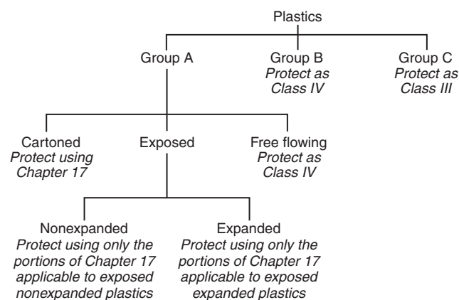
FIGURE 17.1.2.1 Decision Tree.
