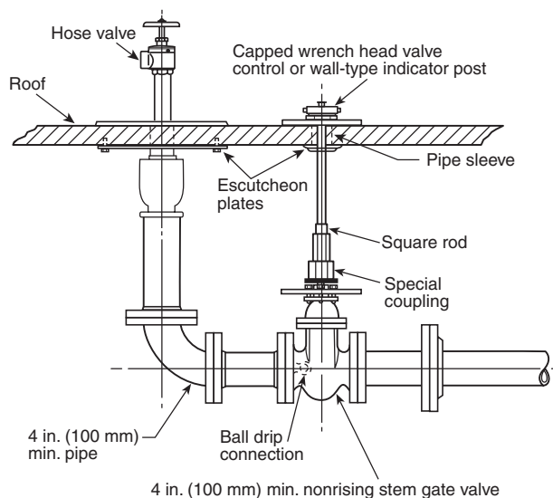
ELEVATION VIEW
