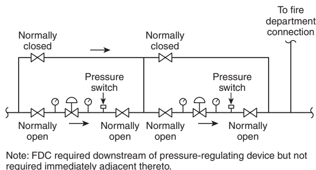
FIGURE A.7.2.4 Dual Pressure-Regulating Device Arrangement.
