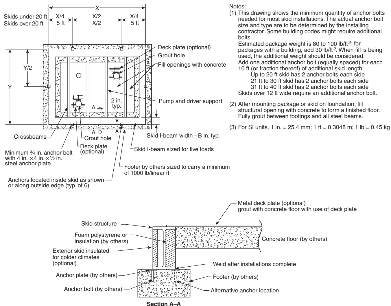
FIGURE A.4.29.9 Typical Foundation Detail for Packaged Fire Pump Assembly.
