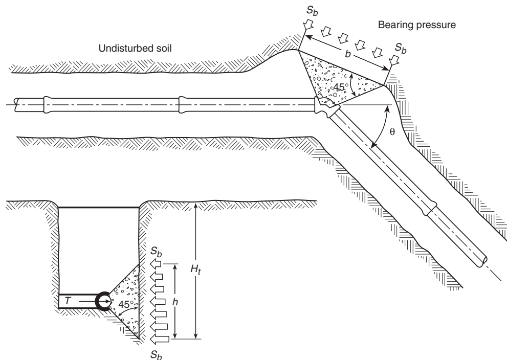
FIGURE A.10.8.2(a) Thrust Forces Acting on Bend.
