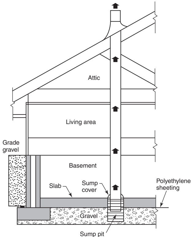
FIGURE 49.2.5.3.4 Passive Radon System Vented Through Sump.
