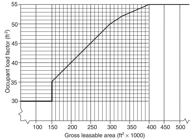
FIGURE 11.3.1.2 Mall Building Occupant Load Factors.
