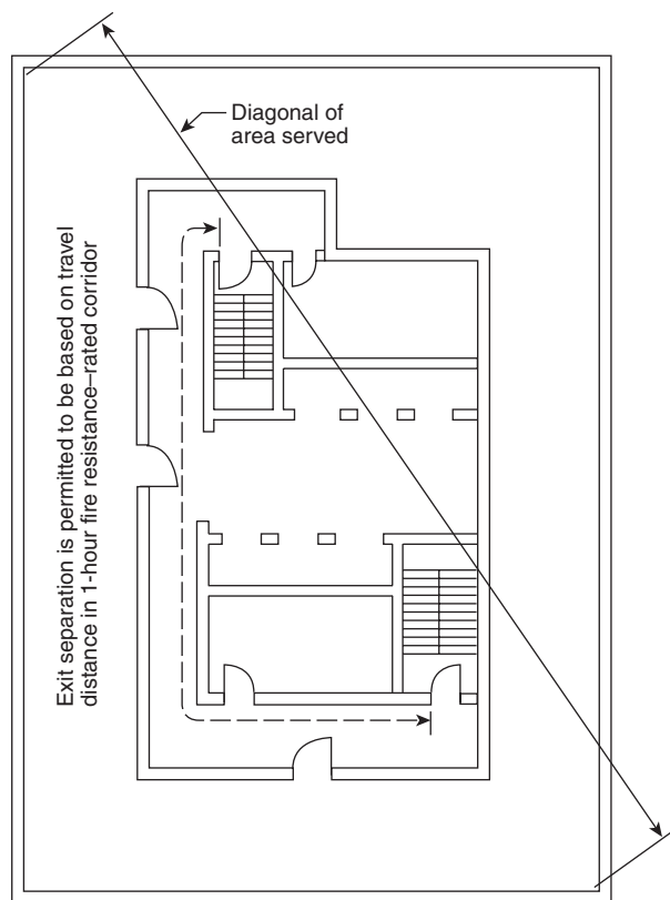
FIGURE A.11.5.1.4.4 Exit Separation Measured Along Corridor Path.
