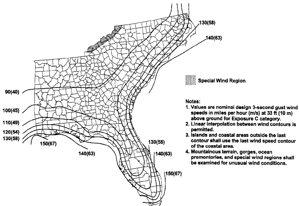
FIGURE A.35.9.2.2(b) Basic Wind Speed — Gulf of Mexico Southeastern U.S. Hurricane Coastline. (Source: Reprinted with permission from ASCE/SEI 7.)
