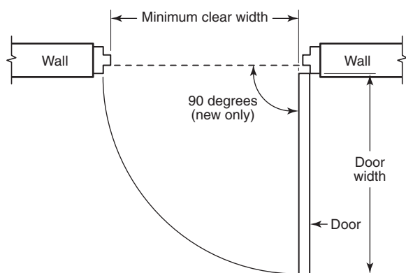
FIGURE A.11.2.1.2.1(a) Minimum Clear Width.
