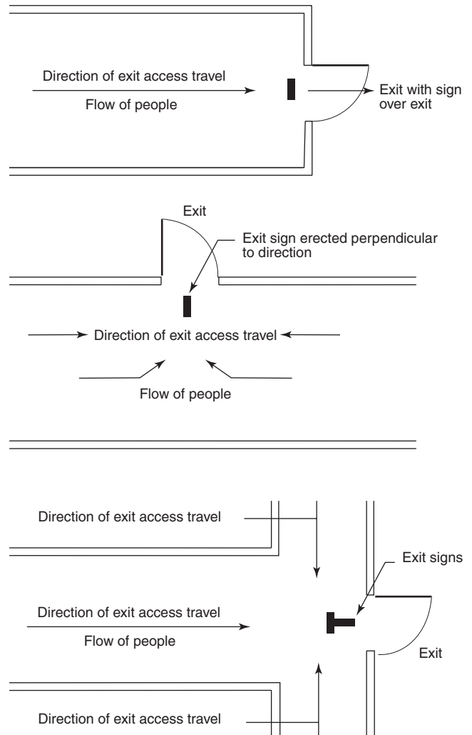
FIGURE A.11.10.1.2.1 Location of Exit Signs.
