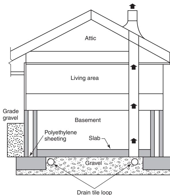
FIGURE 49.2.5.3.5.1 Passive Radon System Using Drain Tile Loop.
