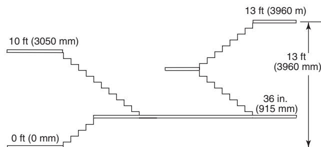
FIGURE A.21.4.4.6.4 Vertical Height Measurement.
