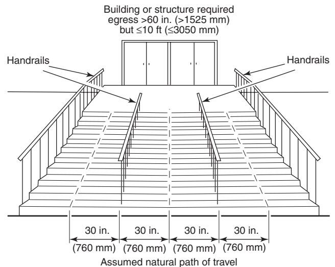
FIGURE A.11.2.2.4.2 Assumed Natural Paths of Travel on Monumental Stairs with Various Handrail Locations.
