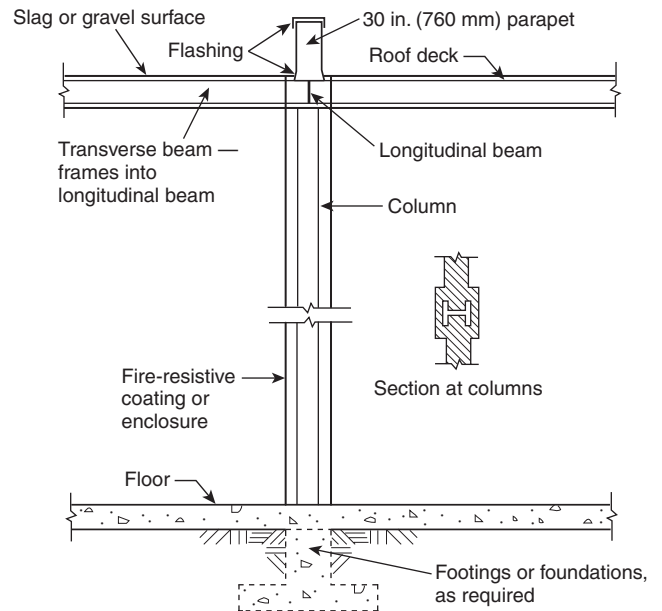
FIGURE A.8.3.2.4(a) Typical Tied HC Fire Wall or Fire Wall Used with Continuous Building Framework. [221: Figure A.5.4(a)]
