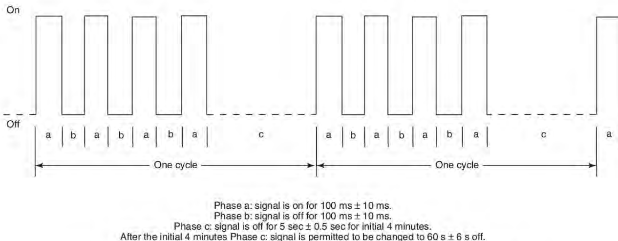
FIGURE 18.4.3.2 Temporal Pattern Parameters — Carbon Monoxide Signal.
