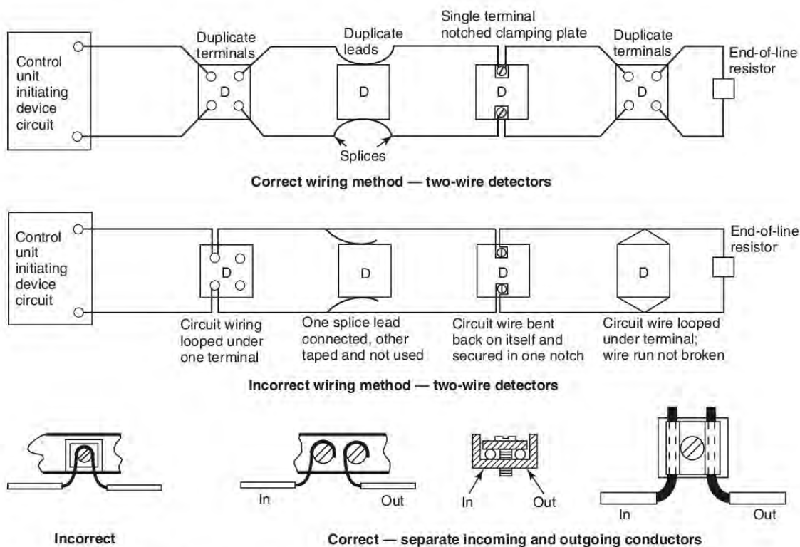
FIGURE A.17.4.6(a) Correct (and Incorrect) Wiring Methods.
