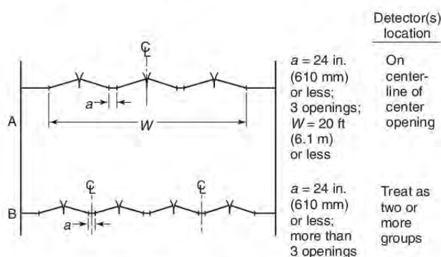
FIGURE 17.7.6.4.3(B) Detector(s) Location \pm 24 in. (610 mm) Requirements for Group Doorways.
