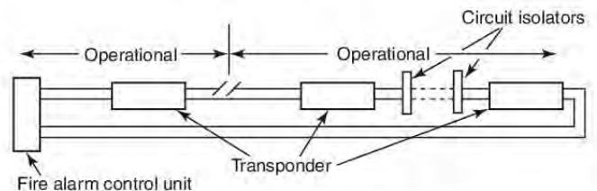
FIGURE F.3.13 Class A with Circuit Isolators.
