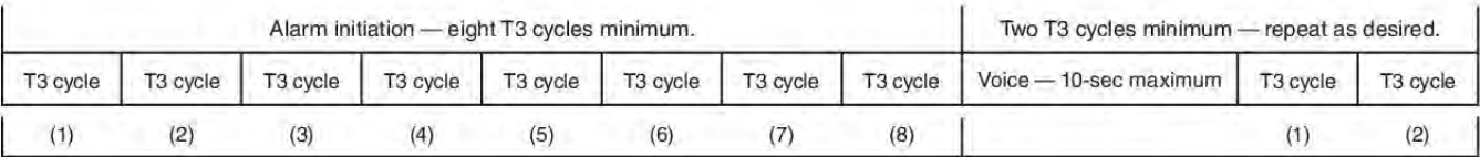
FIGURE A.29.5.5(a) Temporal Pattern Parameters with Eight T3 Cycles Minimum with 10-Second Voice Allowance.
