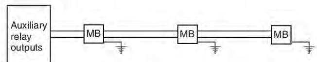
FIGURE F.2.17 Auxiliary Circuit Connected to Municipal Fire Alarm Master Box.
