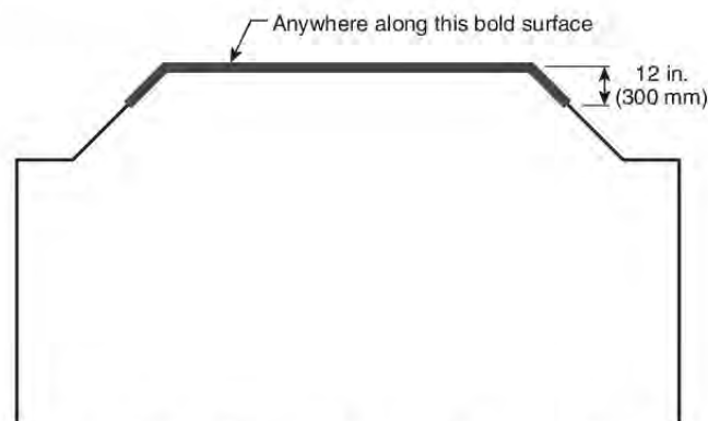
FIGURE A.29.11.3.4(11) Locations Permitted for Smoke Alarms and Smoke Detectors on Tray-Shaped Ceilings.
