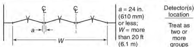
FIGURE 17.7.6.4.3(C) Detector(s) Location \pm 24 in. (610 mm) Requirements for Group Doorways over 20 ft (6.1 m) in Width.
