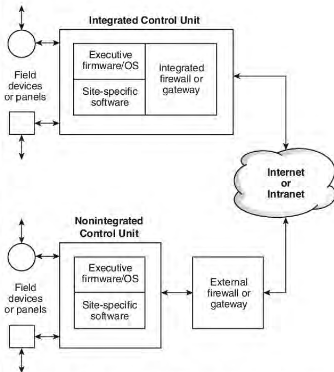
FIGURE J.6.2 System Typical Firewall/Gateway Operation.
