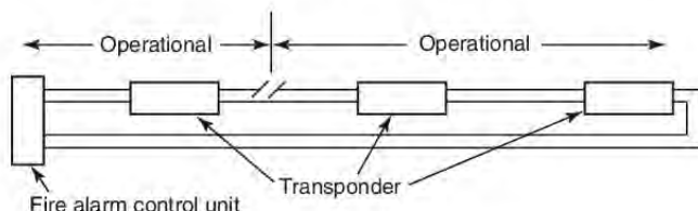
FIGURE F.3.11.1 Class A (Formerly Style 5.0).
