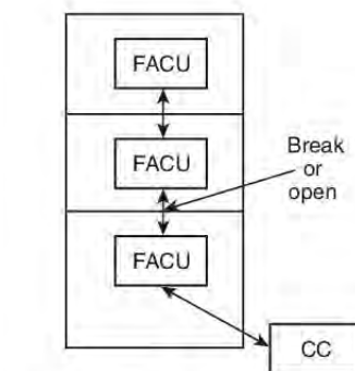
FIGURE E.3.14(f) Style 4 Fiber Network.
