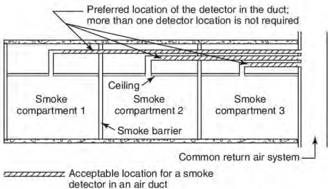
FIGURE A.17.7.6.4.2(c) Detector Location in Duct that Passes Through Smoke Compartments Not Served by Duct.
