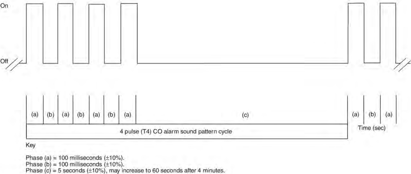
FIGURE A.29.5.4 Four-Pulse Temporal Pattern.
