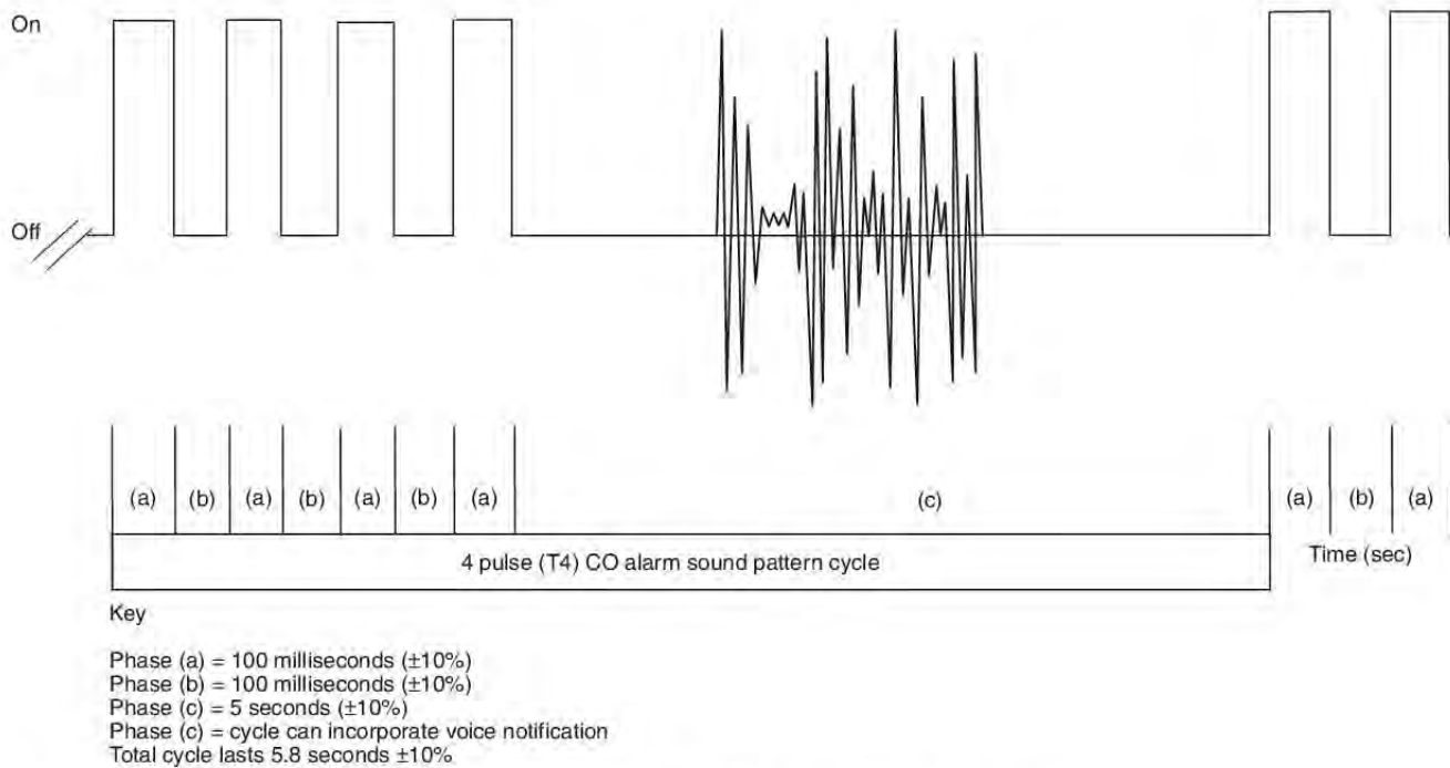
FIGURE A.29.5.6(b) T4 Temporal Pattern Parameters with 1.5-second Voice Allowance.
