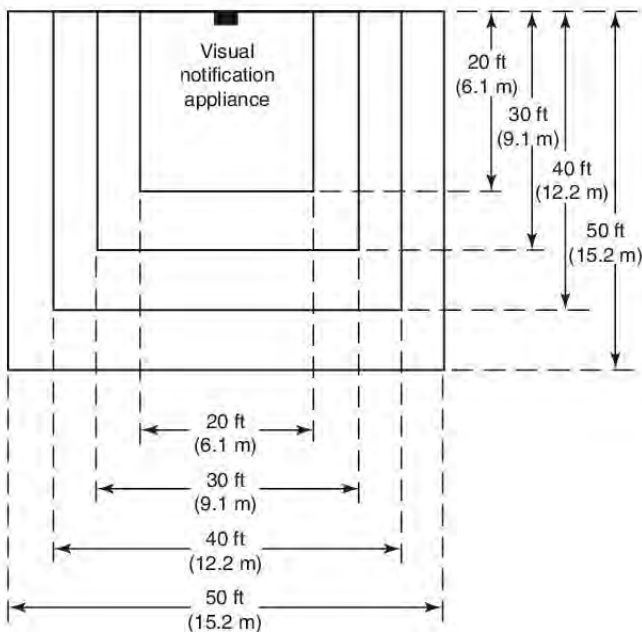
FIGURE 18.5.5.7.1 Room Spacing for Wall-Mounted Visual Notification Appliances.
