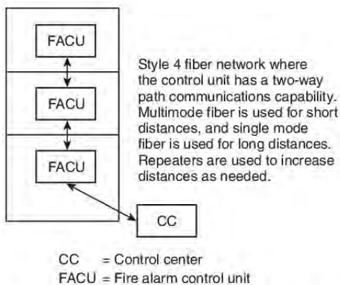
FIGURE E.3.14(f) Style 4 Fiber Network.
