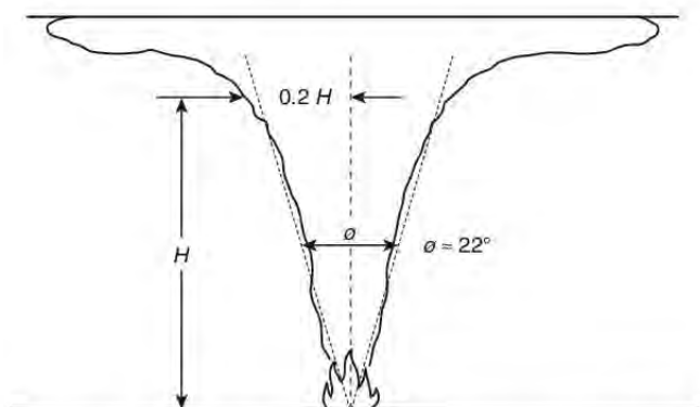
FIGURE A.17.7.4.7.2 The Plume Divergence of an Unconstrained Fire.
