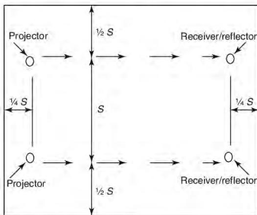
FIGURE A.17.7.4.7 Maximum Distance at Which Ceiling-Suspended Light Projector and Receiver/Reflector Can Be Positioned from End Wall Is One-Quarter Selected Spacing ( S ).
