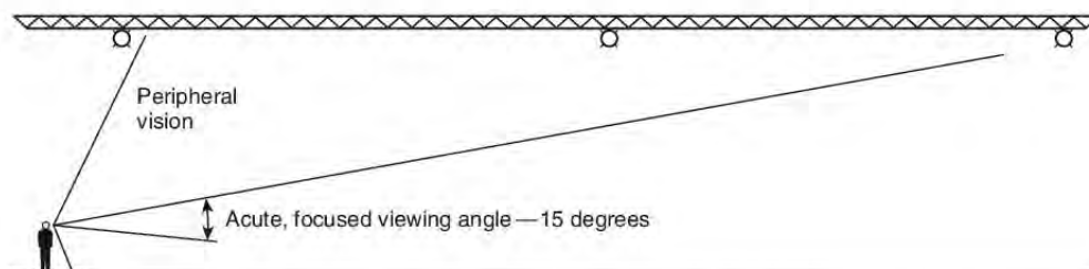
FIGURE A.18.5.4(a) Extended Cone of Vision. (Source: R. P. Schifiliti Associates, Inc.)
