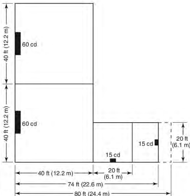
FIGURE A.18.5.5.7(b) Spacing of Wall-Mounted Visual Notification Appliances in Rooms.
