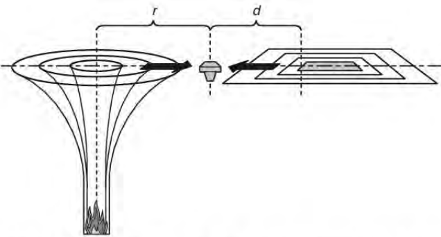
FIGURE B.4.9.1(b) Ceiling Jet Flow in Opposition to Flow from HVAC System.
