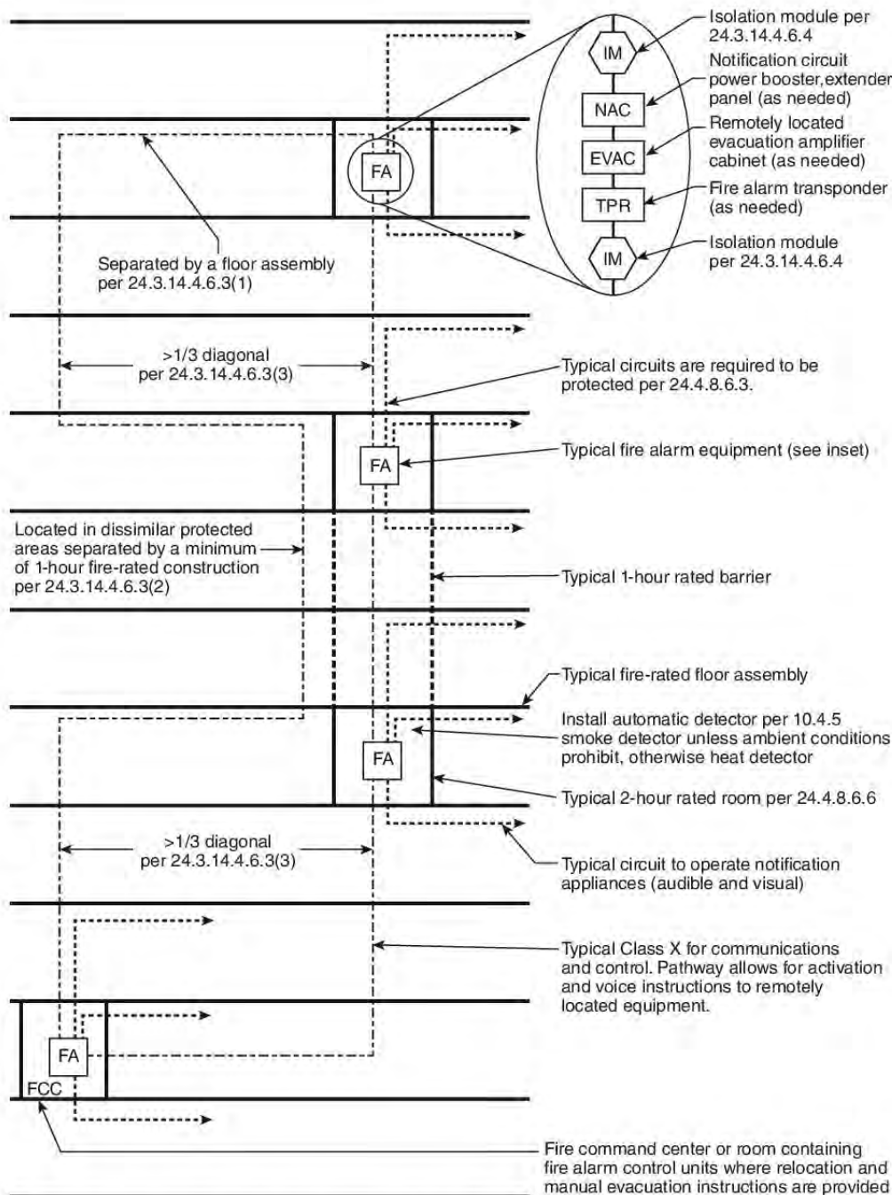
FIGURE A.24.3.14.4.6.3 Simplified Riser Diagram for a High-Rise Building with Relocation or Partial Evacuation.
