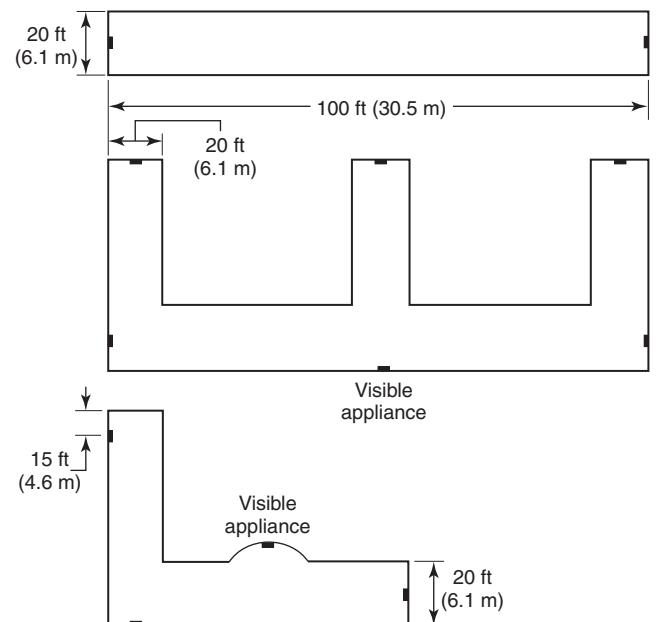
FIGURE A.6.5.5.5 Corridor Spacing for Visible Appliances. [72:Figure A.18.5.5.5]
