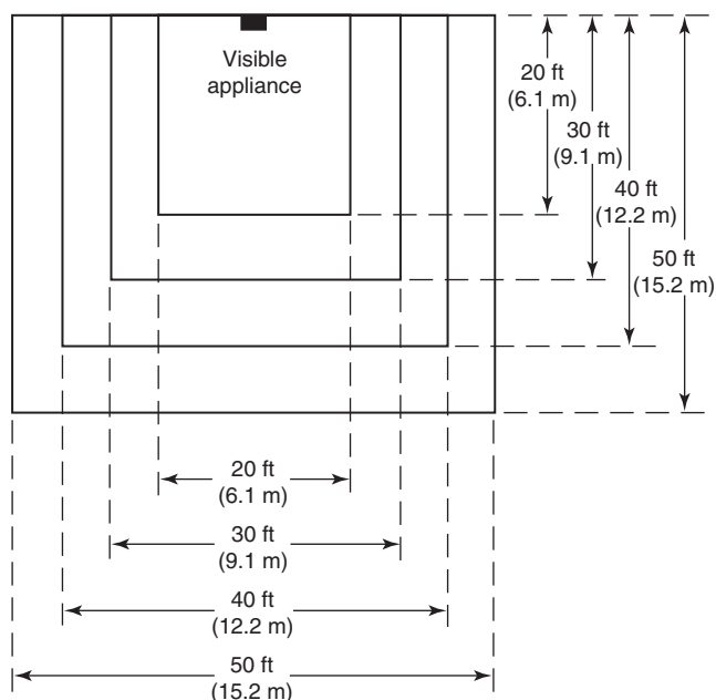
FIGURE 6.5.5.4.1 Room Spacing for Wall-Mounted Visible Appliances. [72:Figure 18.5.5.4.1]
