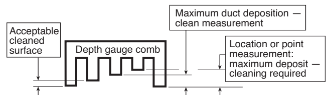
FIGURE 11.6.1.1.2 Depth Gauge Comb.
