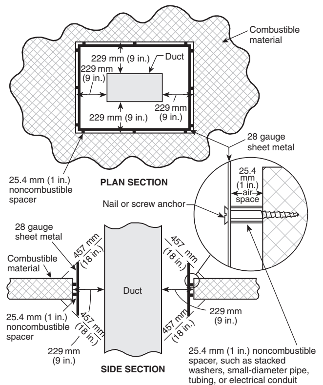
FIGURE A.4.2(g) Example of Clearance Reduction System: 229 mm (9 in.) Clearance to Combustible Material.
