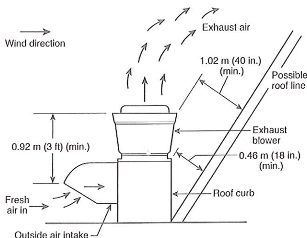
FIGURE 7.8.2.1 Upblast Fan Clearances.
