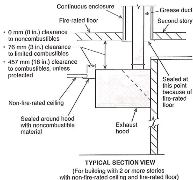
FIGURE A.4.2(e) Detail Drawings Showing Hoods Penetrating Ceilings.
