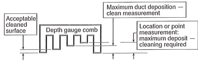
FIGURE A.11.6.2 Depth Gauge Comb.
