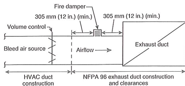
FIGURE A.8.4.1 System for Introducing Bleed Air into a Master Exhaust Duct.
