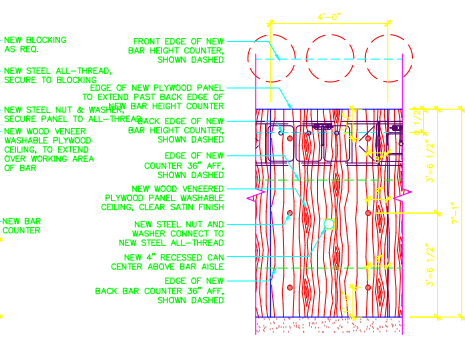
D5 ENLARGED CEILING PANEL — BAR
