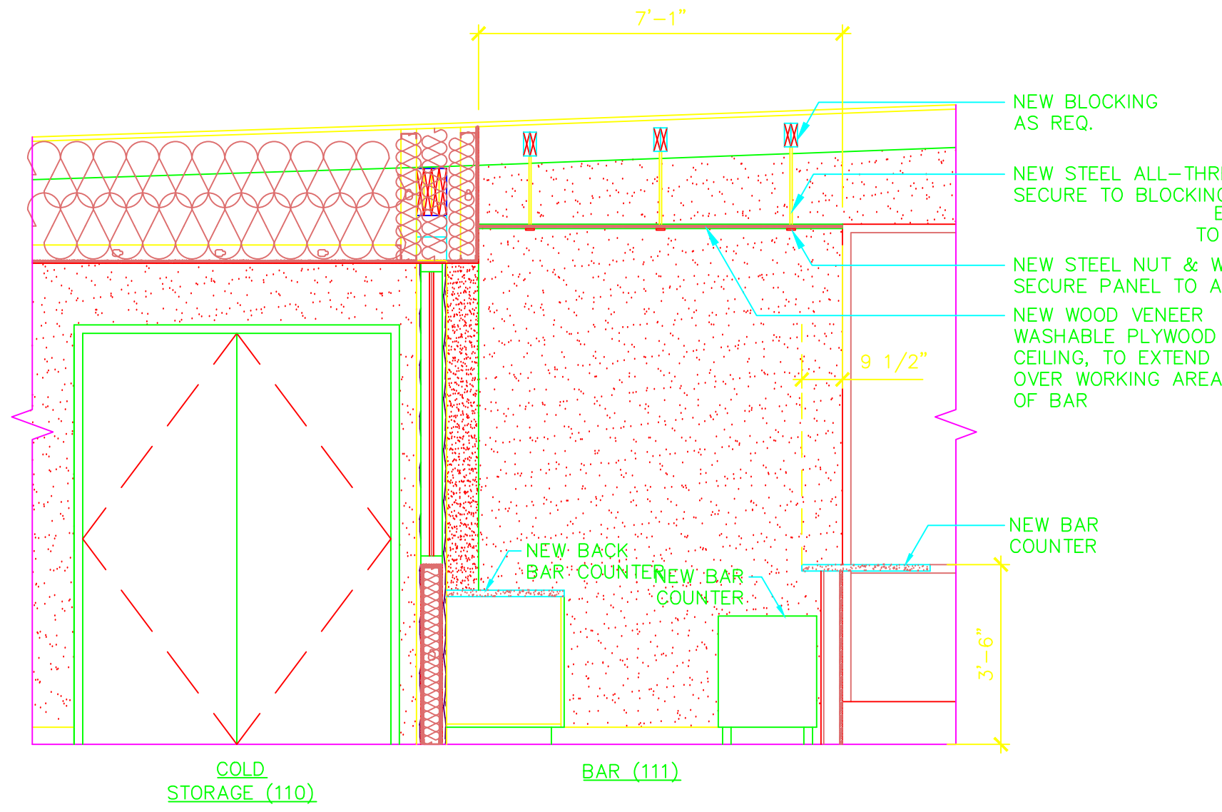
D3 ENLARGED SECTION - BAR (111) 3/8" = 1'-0"
