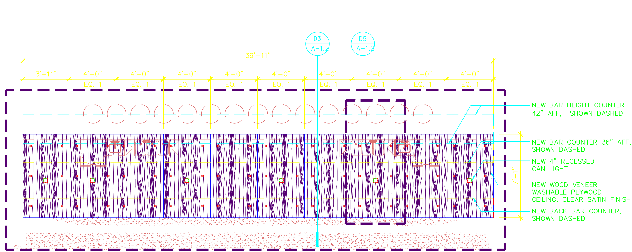
D1 ENLARGED REFLECTED CEILING - BAR (111) 1/4" = 1'-0"
