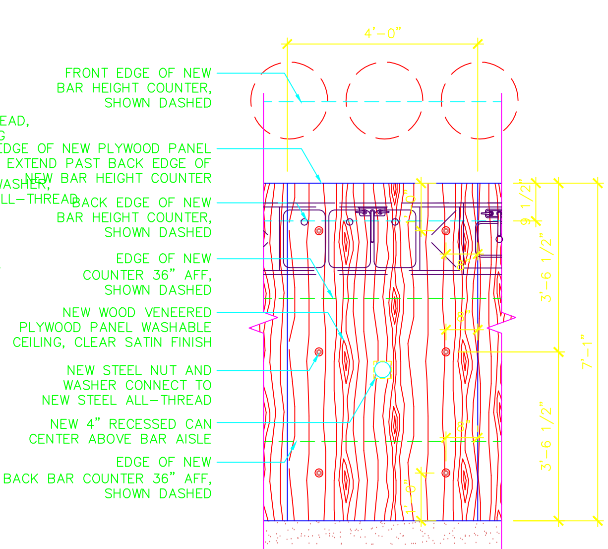
D5 ENLARGED CEILING PANEL - BAR (111) 1/2" = 1'-0"
