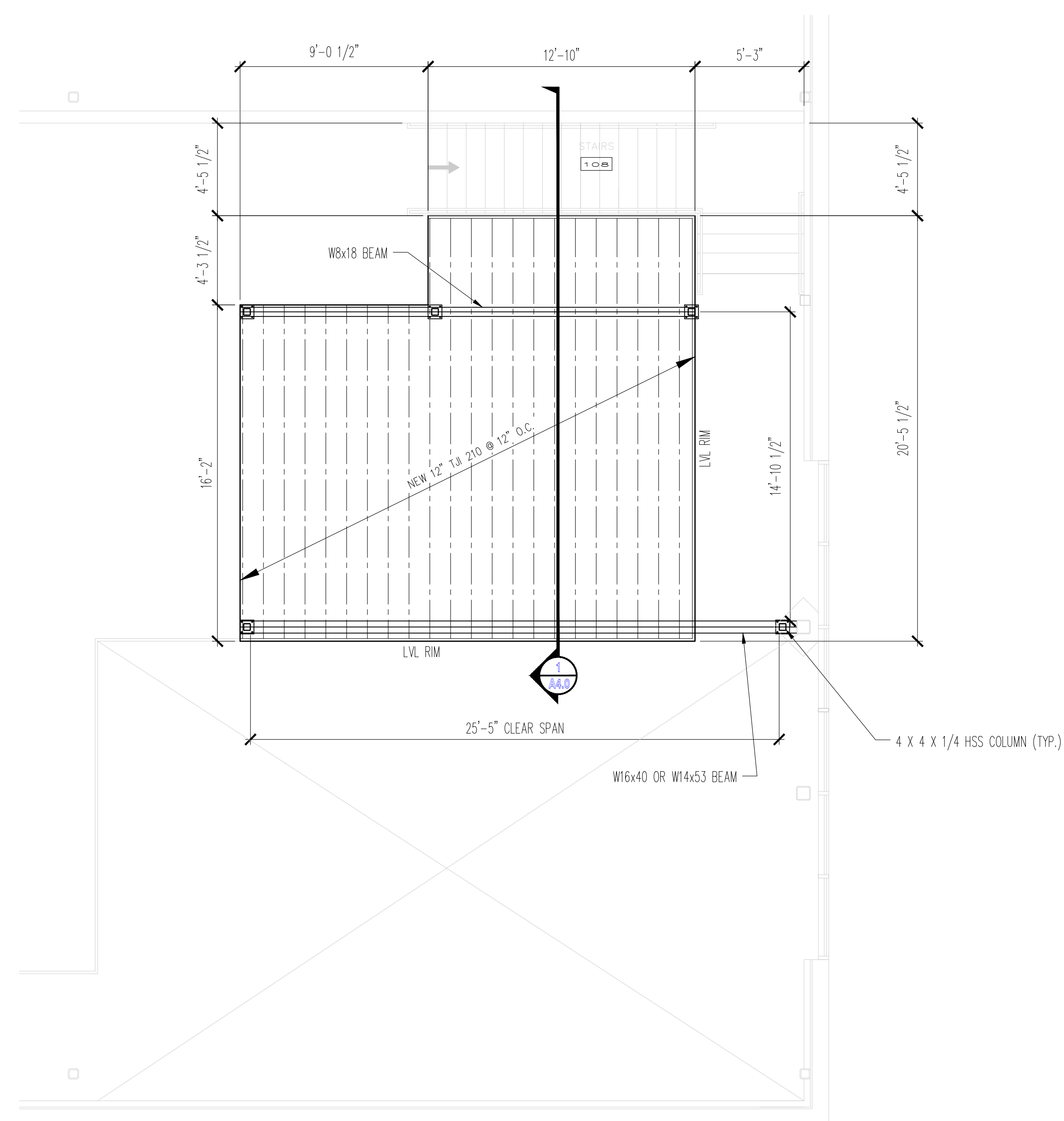
UPPER LEVEL FLOOR FRAMING PLAN
