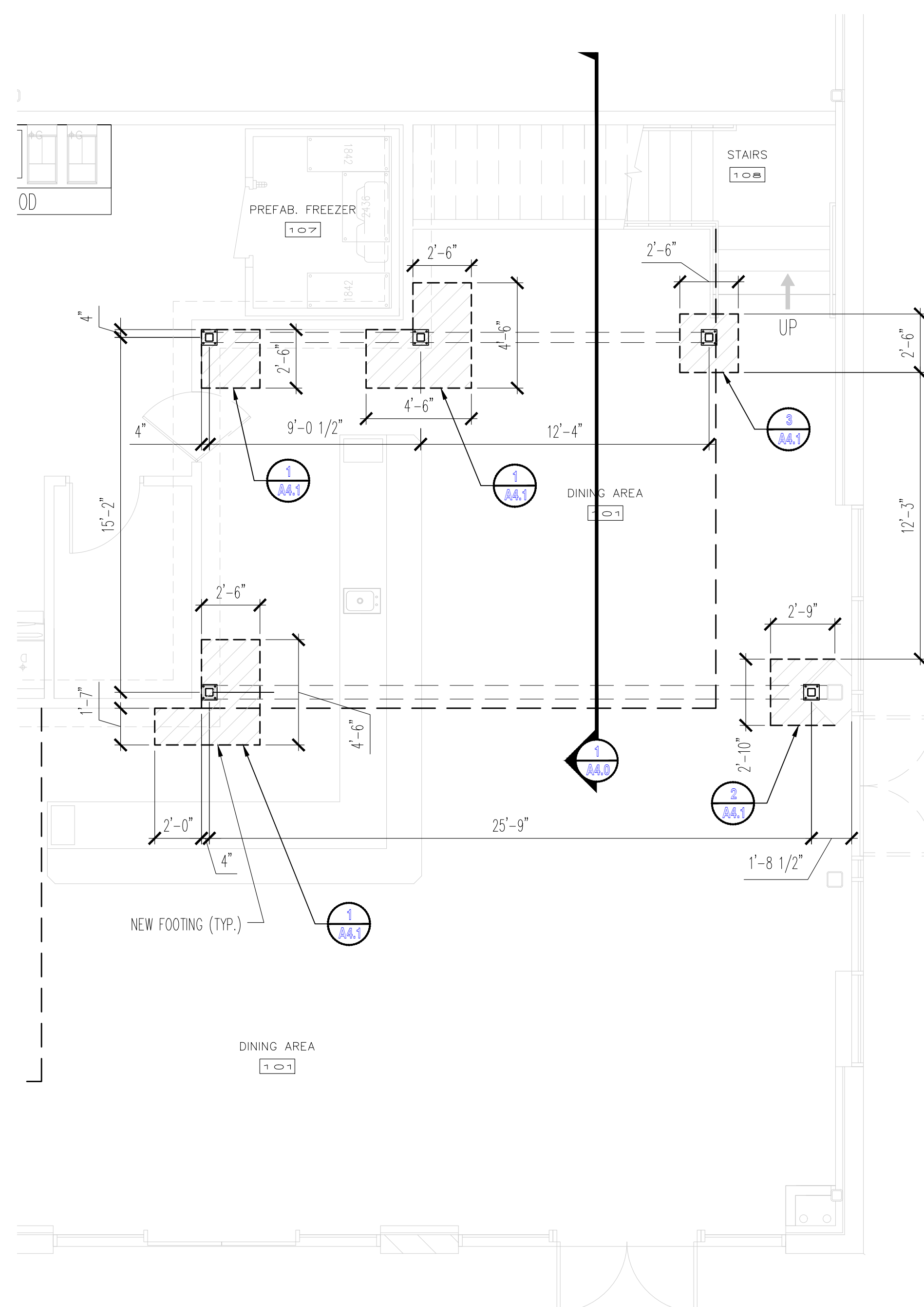
FOOTING PLAN
