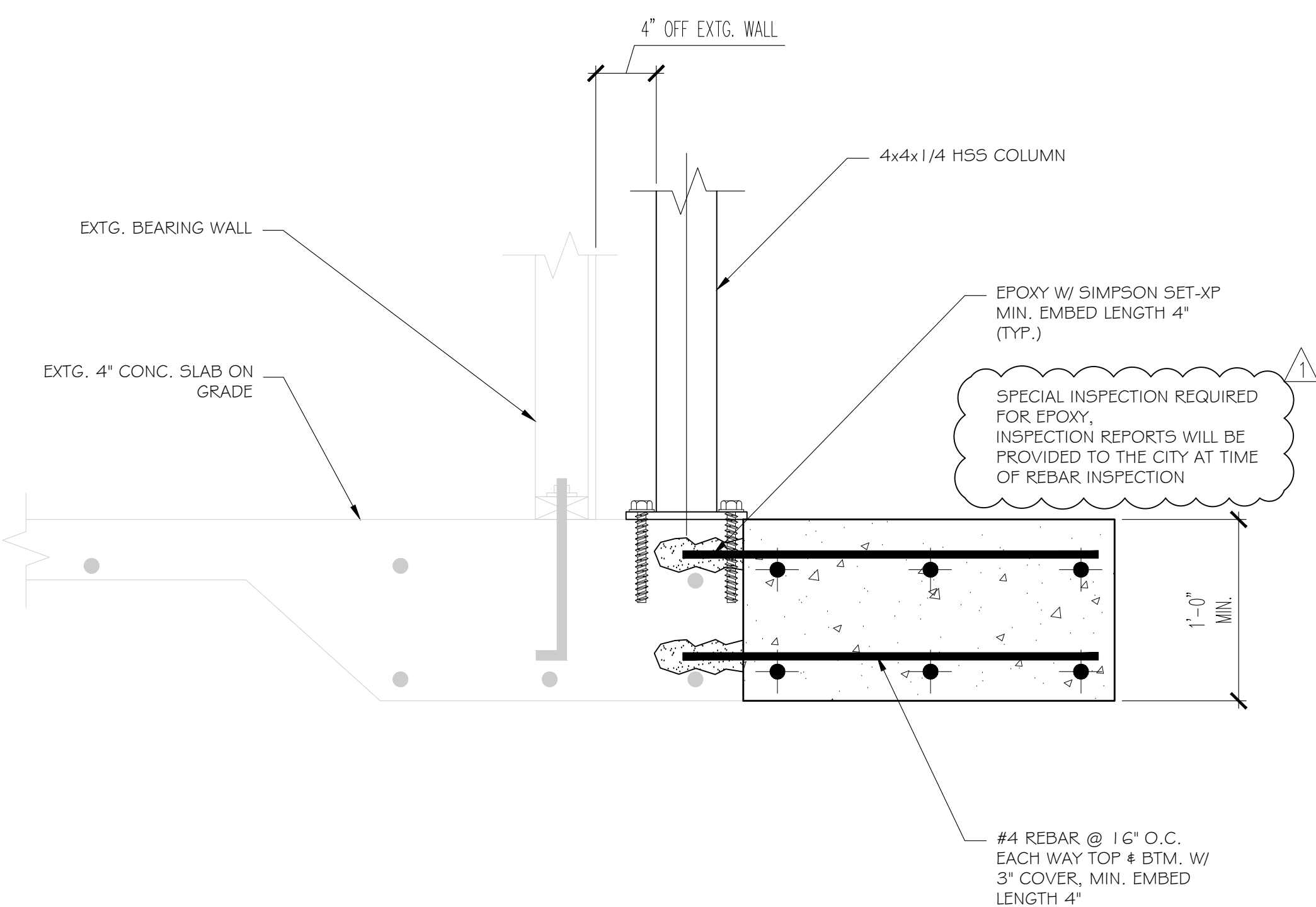
FOUNDATION DETAIL AT INTERIOR WALL
