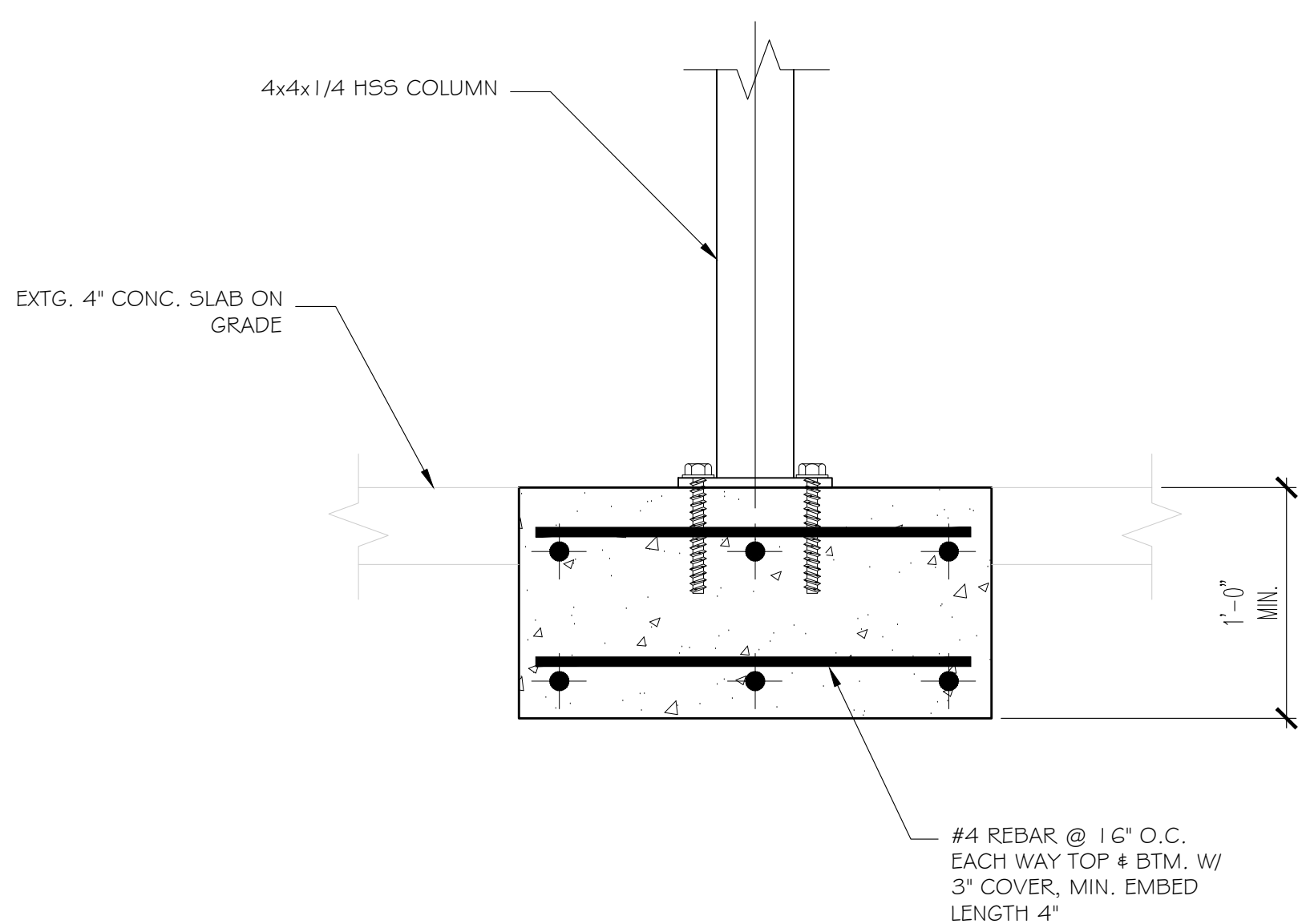
FOUNDATION DETAIL AT STAIRS
