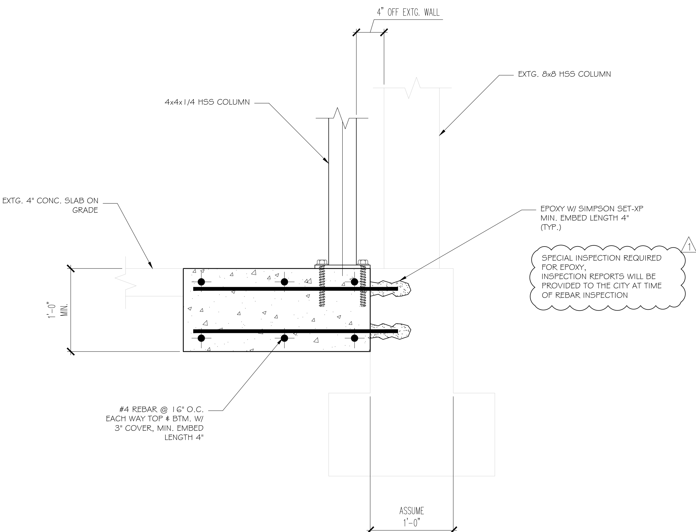
FOUNDATION DETAIL AT EXTERIOR WALL
