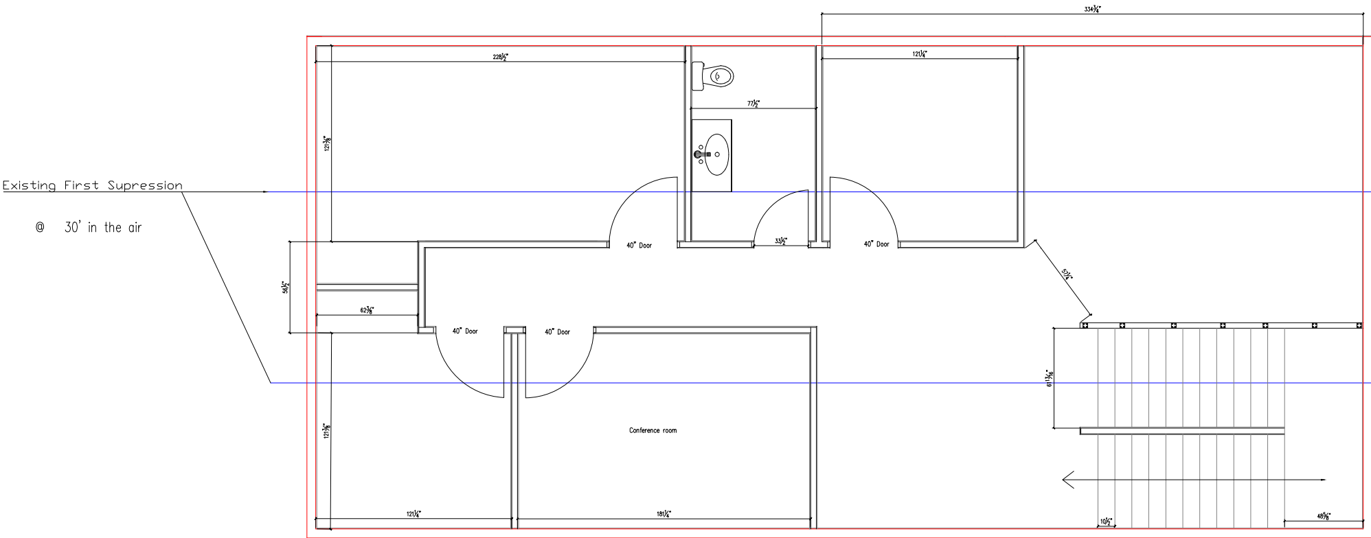
Second Floor
