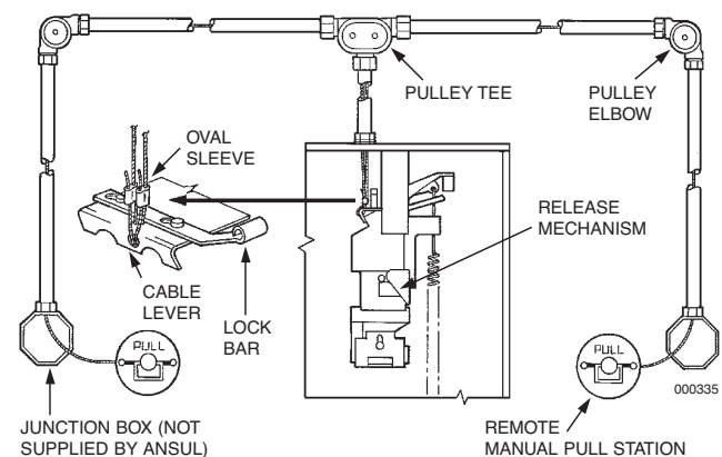
REMOTE MANUAL PULL STATION DUAL APPLICATION
