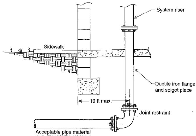
A.10.6.3.1 Riser Entrance Location. [24: Figure A.10.6.3.1]
