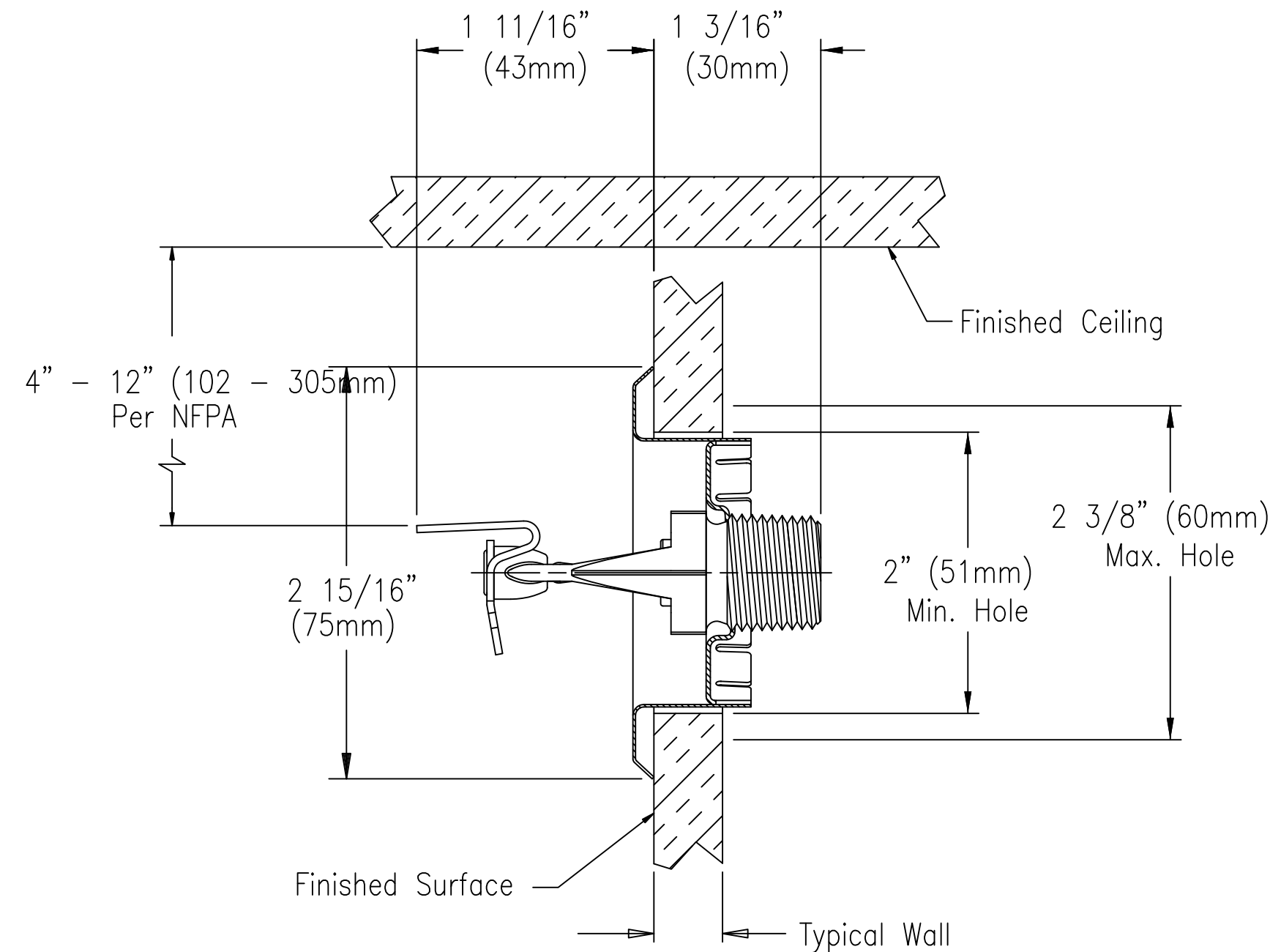
MAXIMUM RECESS
