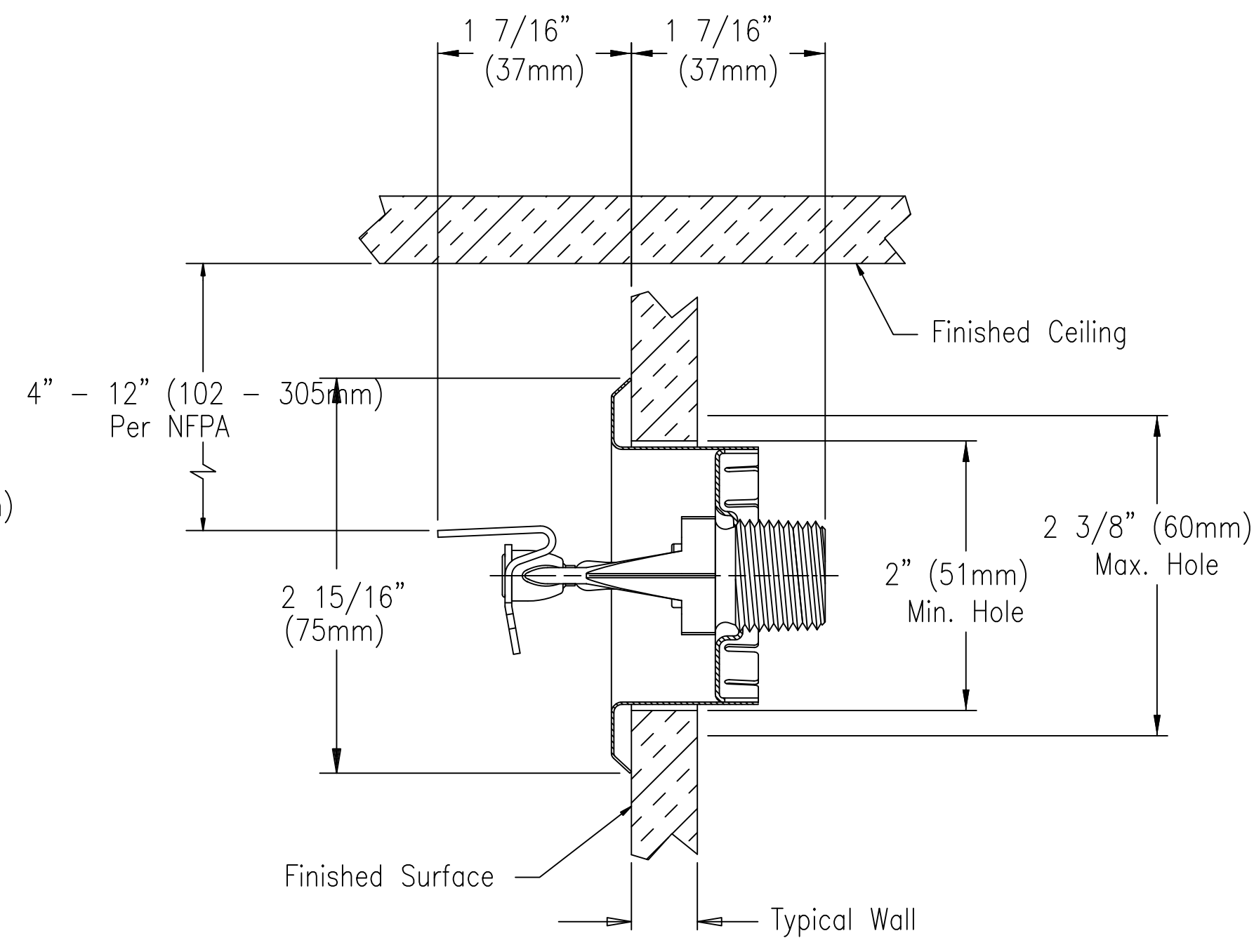
MAXIMUM RECESS
