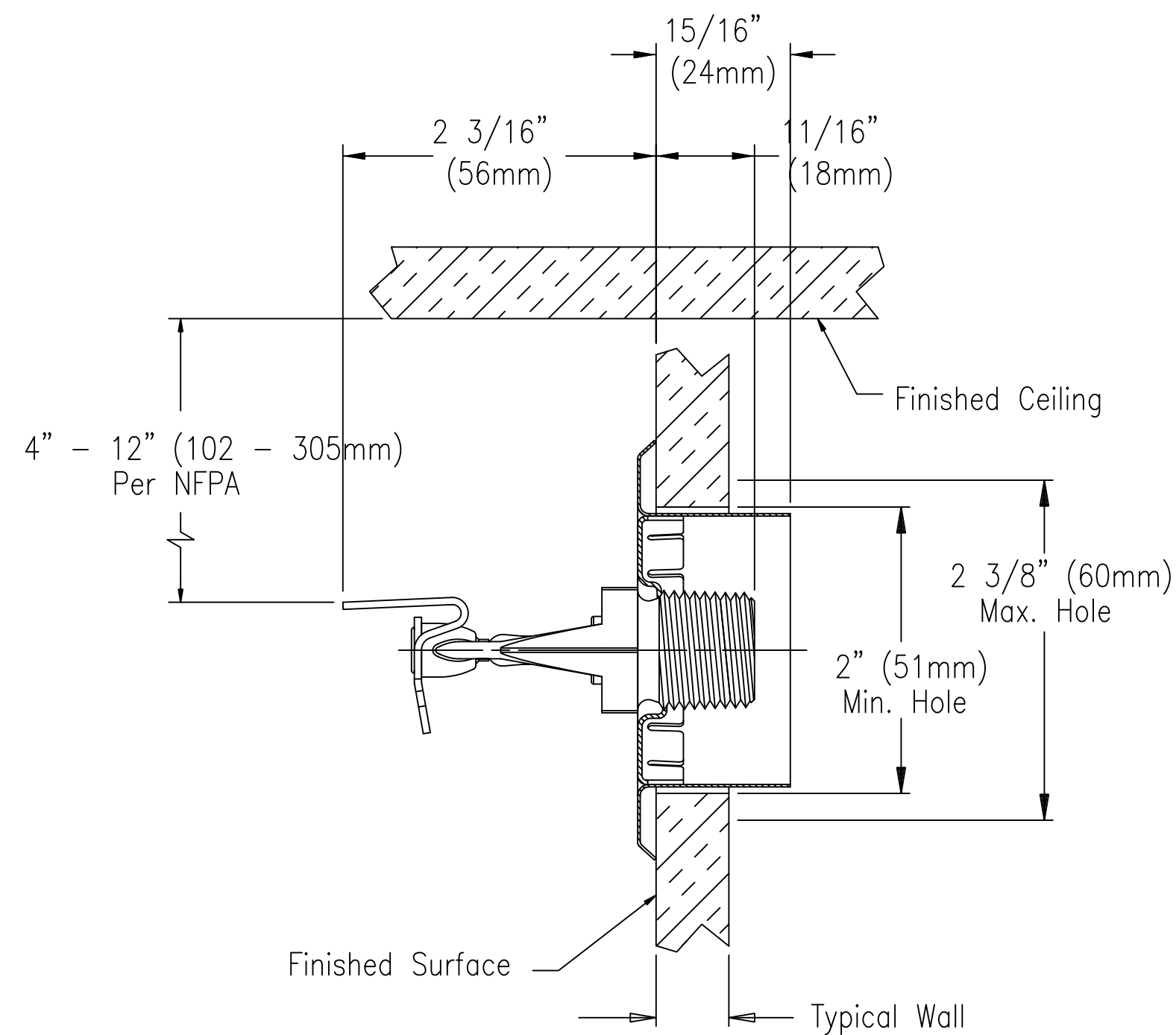
MAXIMUM EXTENSION
