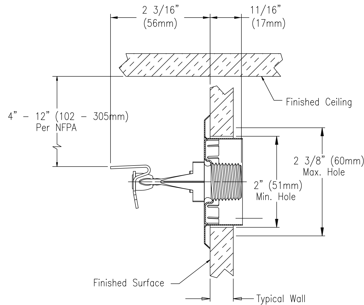
MAXIMUM EXTENSION
