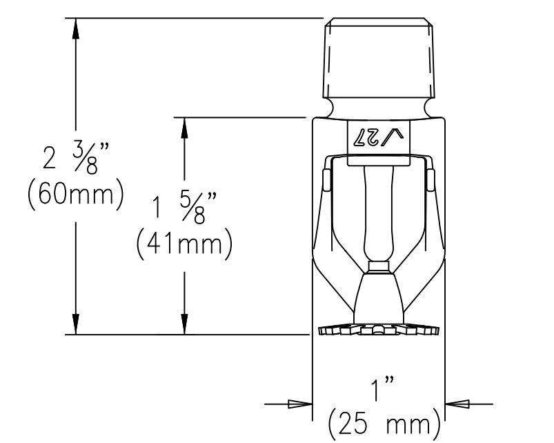
Standard Pendent – V2707, V2708
