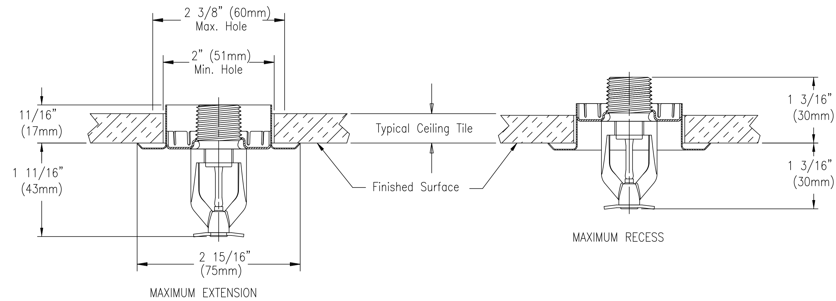
1/2" Adjustment Recessed – V2707, V2708
