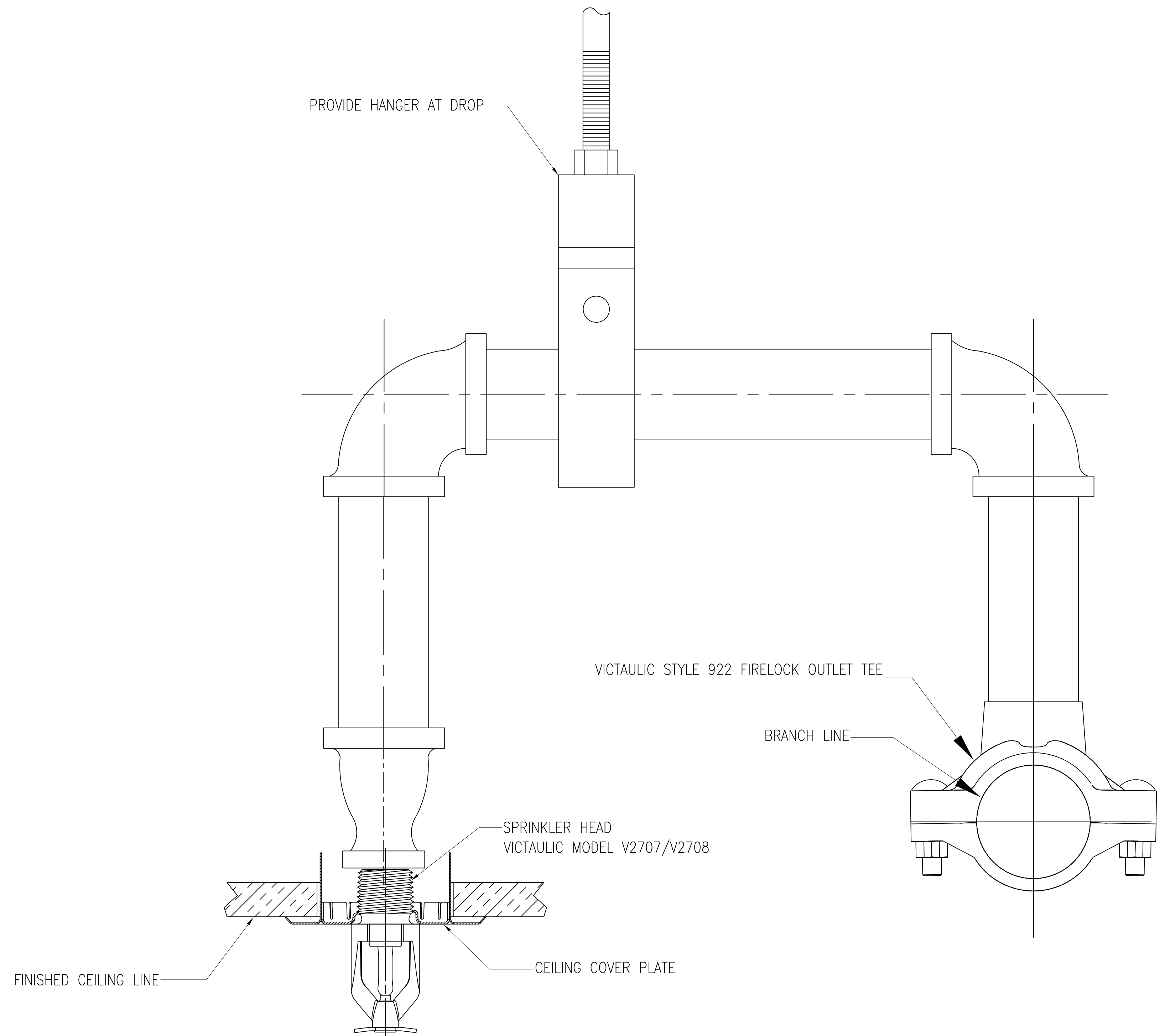
TYPICAL INSTALLATION
