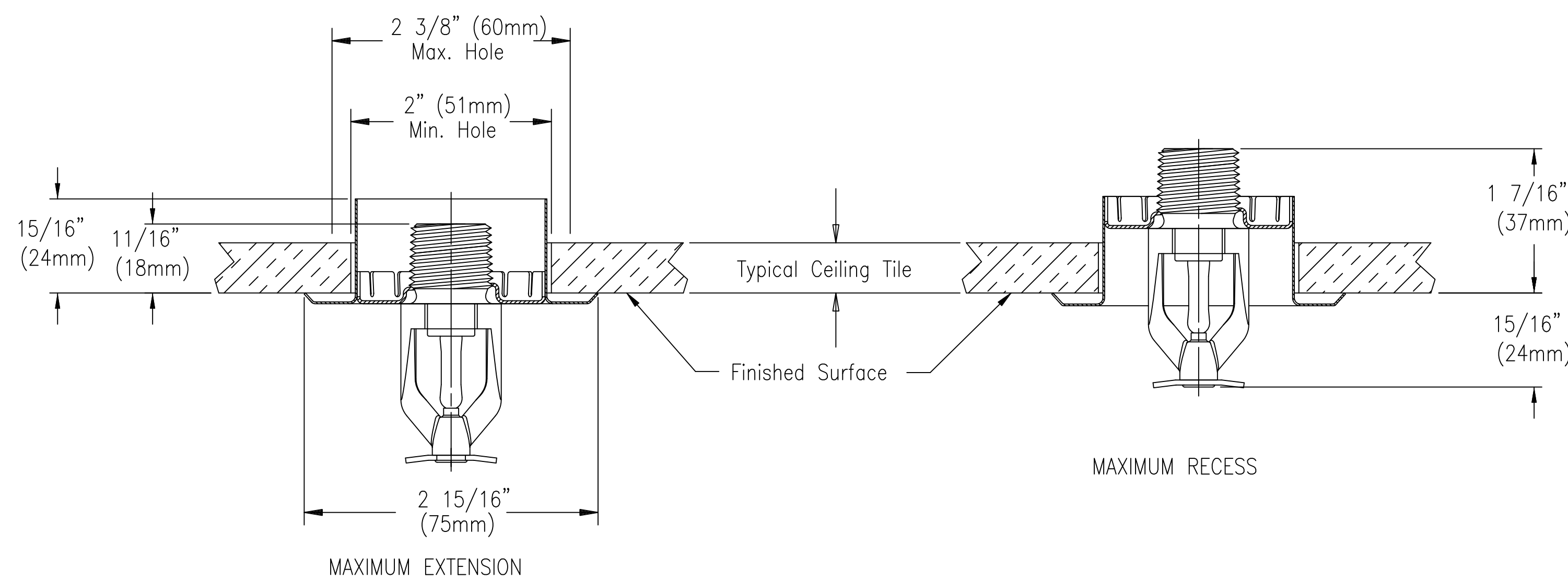
3/4" Adjustment Recessed – V2707, V2708
