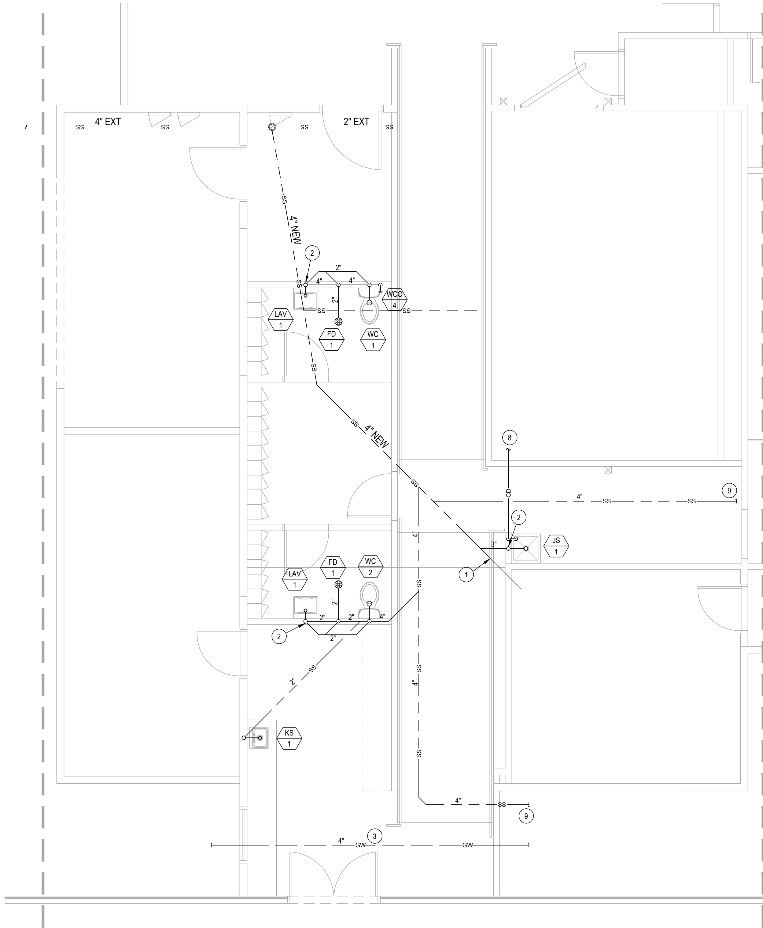
NORTH WASTE AND VENT PLUMBING PLAN SCALE: 1/4"=1'-0"
