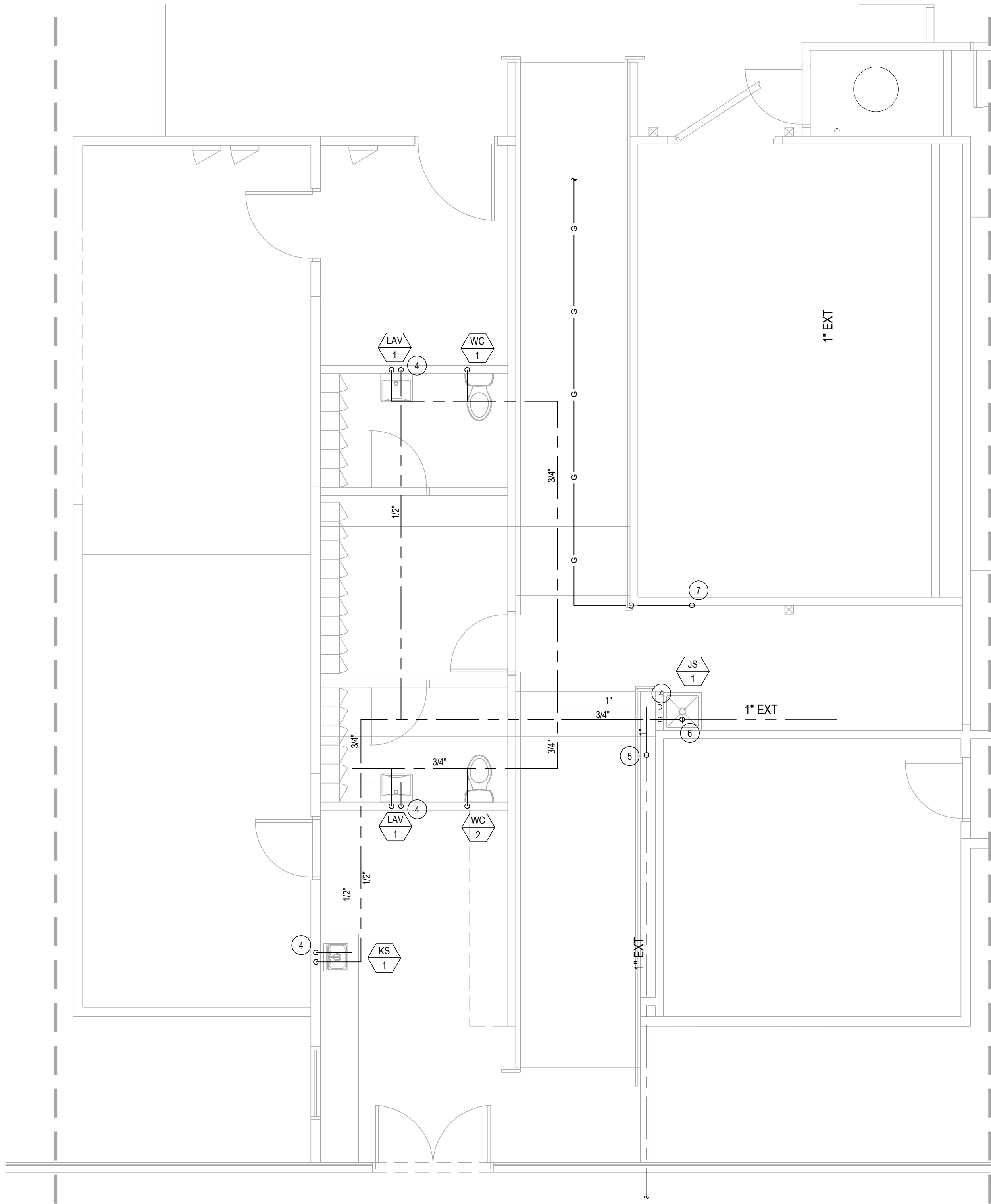
NORTH WATER AND GAS PLUMBING PLAN SCALE: 1/4"=1'-0"
