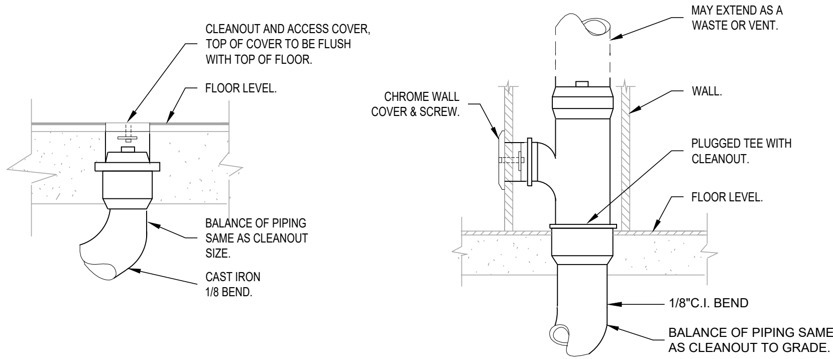
FLOOR CLEAN-OUT
